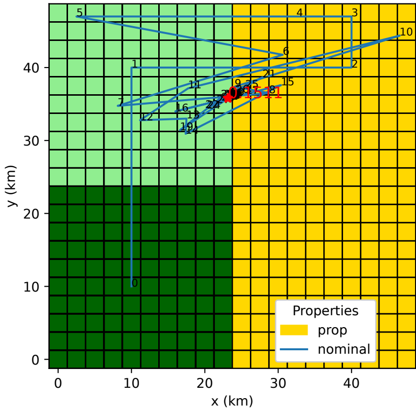
Progression of Nelder-Mead Algorithm over Burn Area
