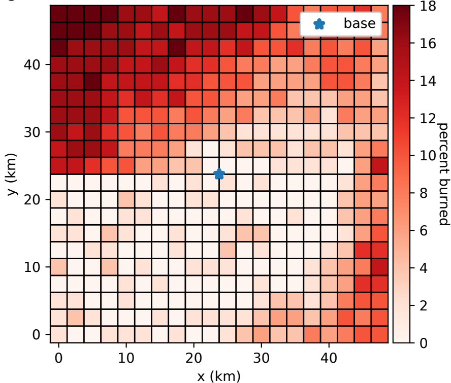
Avg. Burn Area (50 3-Strike Scenarios) for Centered Base
