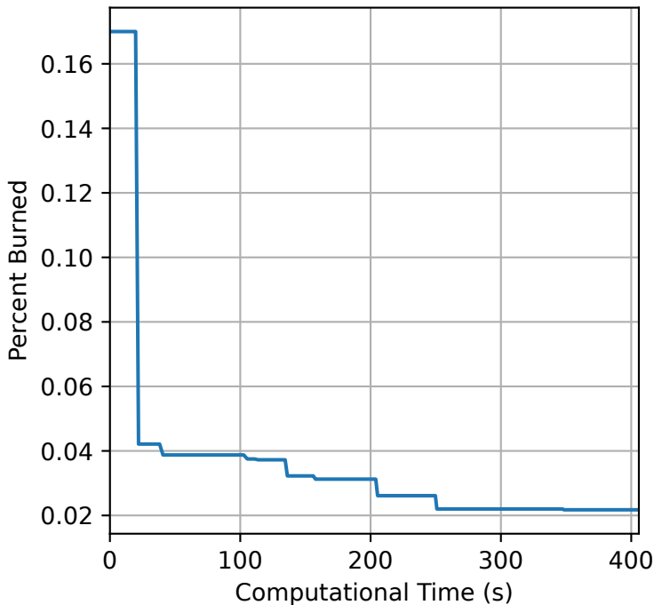
Progression of Direct Algorithm Over Time
