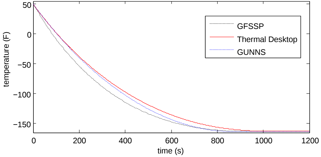
Temperature: Oxygen Tank
