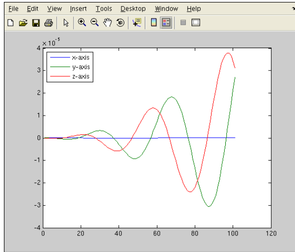
Figure 40.10: The variation with time of the difference between the analytical and numerical solutions for the velocity of B with respect to A.
