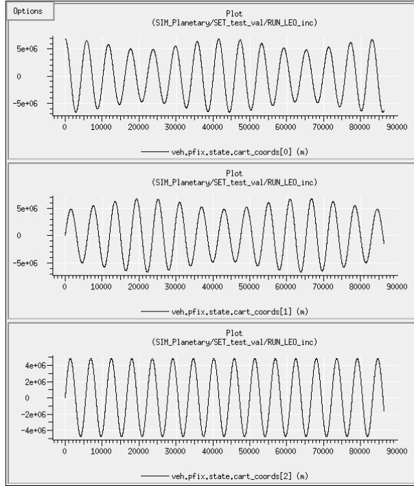
Figure 35.4: The variation of position with time, expressed in Cartesian coordinates.
