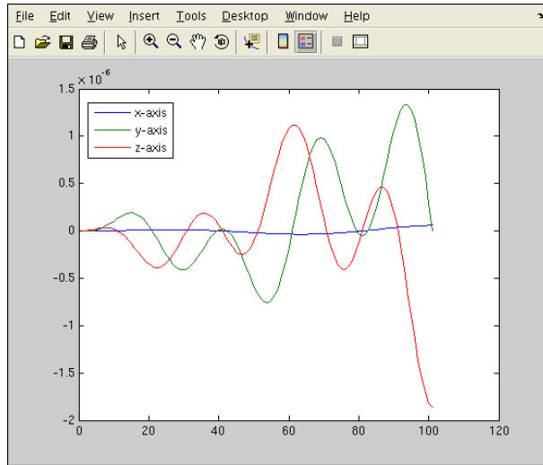
Figure 40.4: The variation with time of the difference between the analytical and numerical solutions for the position of B with respect to A.
