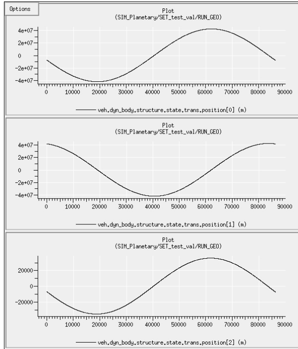
Figure 35.14: The variation of position with time, expressed in inertial coordinates.
