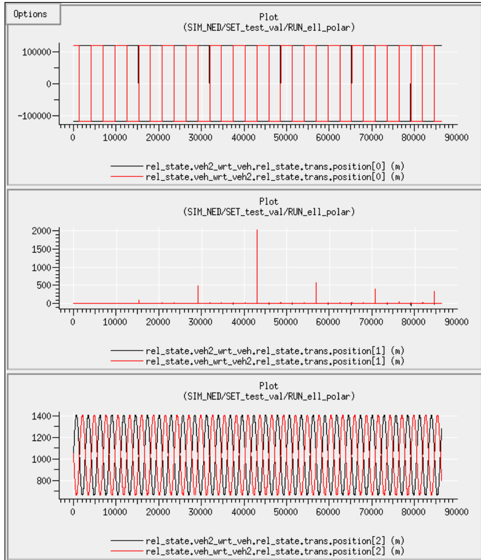
Figure 25.2: The relative states for a polar orbit, with elliptical geometry used to define the reference frame.
