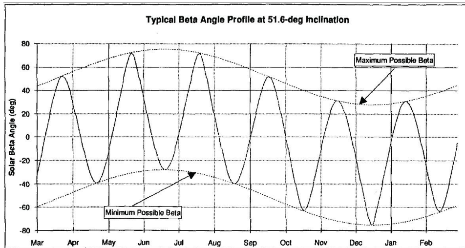
Figure 43.2: The variation with time of the Solar Beta angle for an orbit with inclination of 51.6 degrees. The high frequency oscillation is due to precession, and the long period variation due to Earth's motion around Sun.
