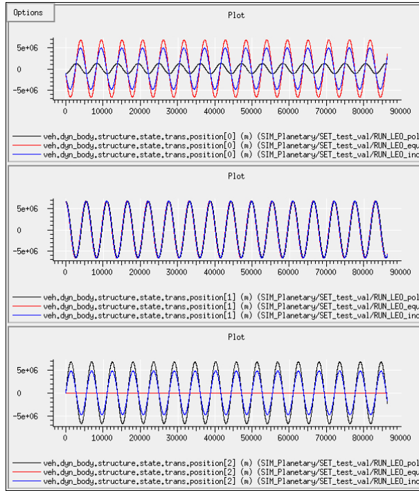
Figure 35.8: The variation of position with time, expressed in inertial coordinates.
