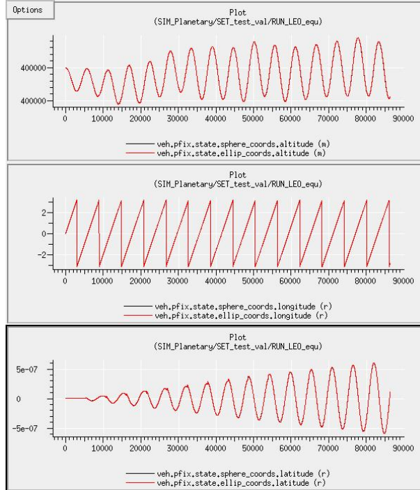
Figure 35.3: The variation of position with time, expressed in Altitude-Longitude-Latitude coordinates, both spherical and elliptical (geodetic).
