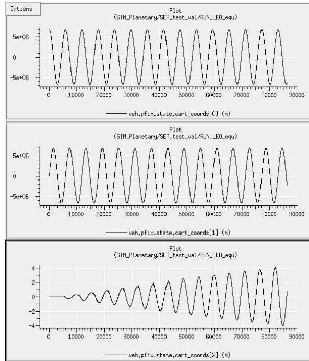
Figure 35.1: The variation of position with time, expressed in Cartesian coordinates.
