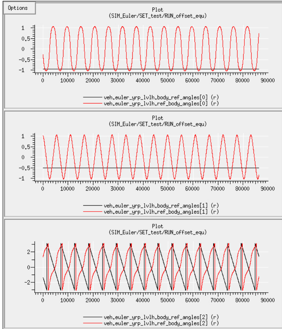
Figure 10.4: The Euler angles for the case in which the LVLH frame and body frame were initially un-aligned, and rotating with respect to each other on the pitch axis of the LVLH reference frame. Angles are expressed in a Yaw-Roll-Pitch sequence. Notice that when Pitch is last in the sequence, the angles associated with the transformation from body frame to LVLH (expressed in body frame) show a similar pattern to that in Figure 10.1, but that is not the case when representing the relative attitude from the LVLH frame to the body frame (this is expressed in the LVLH frame).
