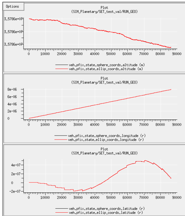
Figure 35.15: The variation of position with time, expressed in Altitude-Longitude-Latitude coordinates, both spherical and elliptical (geodetic).
