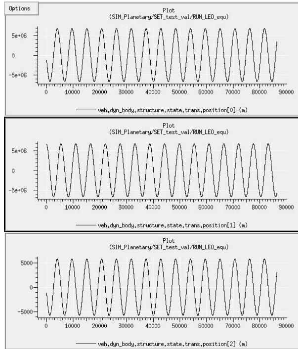
Figure 35.2: The variation of position with time, expressed in inertial coordinates.
