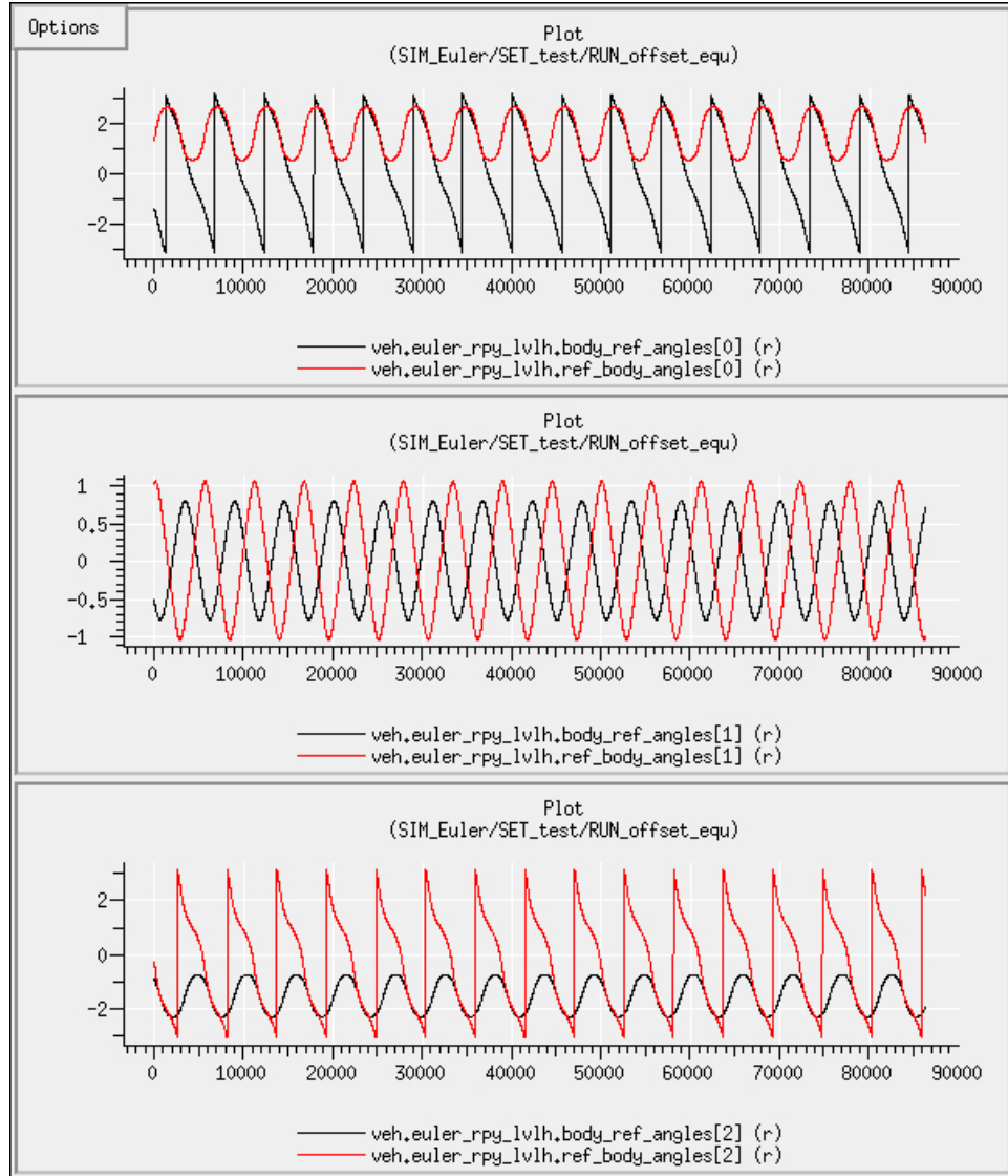
Figure 10.5: The Euler angles for the case in which the LVLH frame and body frame were initially un-aligned, and rotating with respect to each other on the pitch axis of the LVLH reference frame. Notice that the variation is non-sinusoidal, and that the amplitudes differ between the two representations of the transformation.
