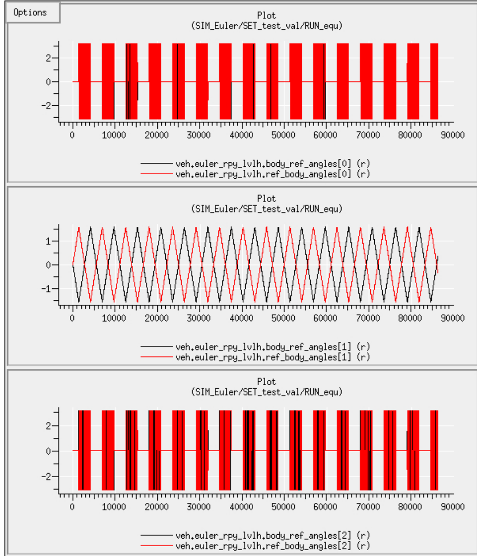
Figure 10.2: The Euler angles for the case in which the LVLH frame and body frame were initially aligned, and rotating with respect to each other on their respective pitch axes, expressed in a Roll-Pitch-Yaw sequence. Notice that the Pitch has a total range of only \pi radians; this is compensated for by the combined effect of adding in \pi rotations on the yaw and roll axes.
