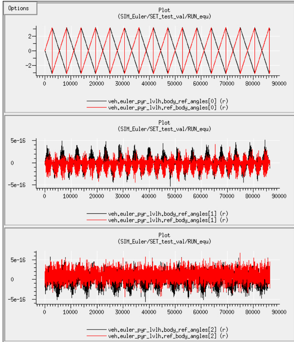
Figure 10.1: The Euler angles for the case in which the LVLH frame and body frame were initially aligned, and rotating with respect to each other on their respective pitch axes, expressed in a Pitch-Yaw-Roll sequence.
