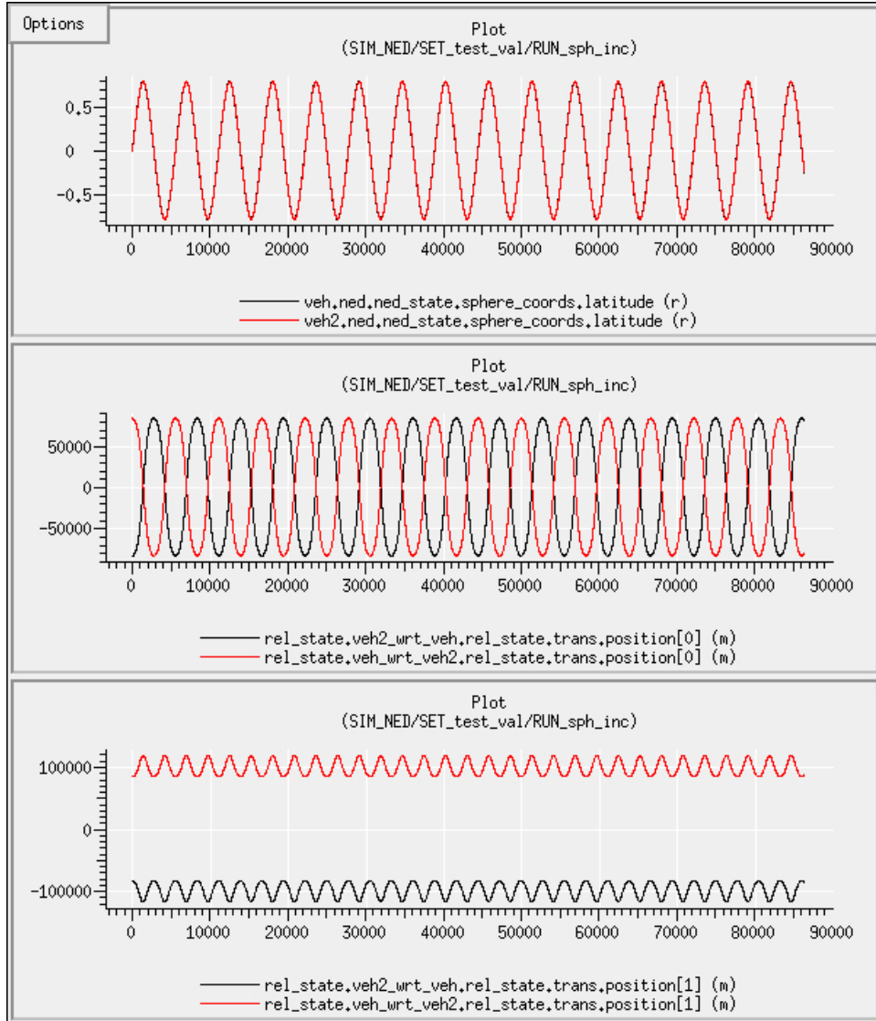
Figure 25.5: The variation with time of latitude and of the North and East components of the relative states for an orbit inclined at 45 degrees, with spherical geometry used to define the reference frame.
