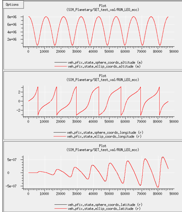
Figure 35.12: The variation of position with time, expressed in Altitude-Longitude-Latitude coordinates, both spherical and elliptical (geodetic).
