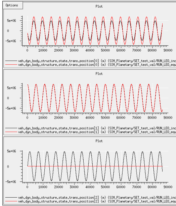
Figure 35.5: The variation of position with time, expressed in inertial coordinates.
