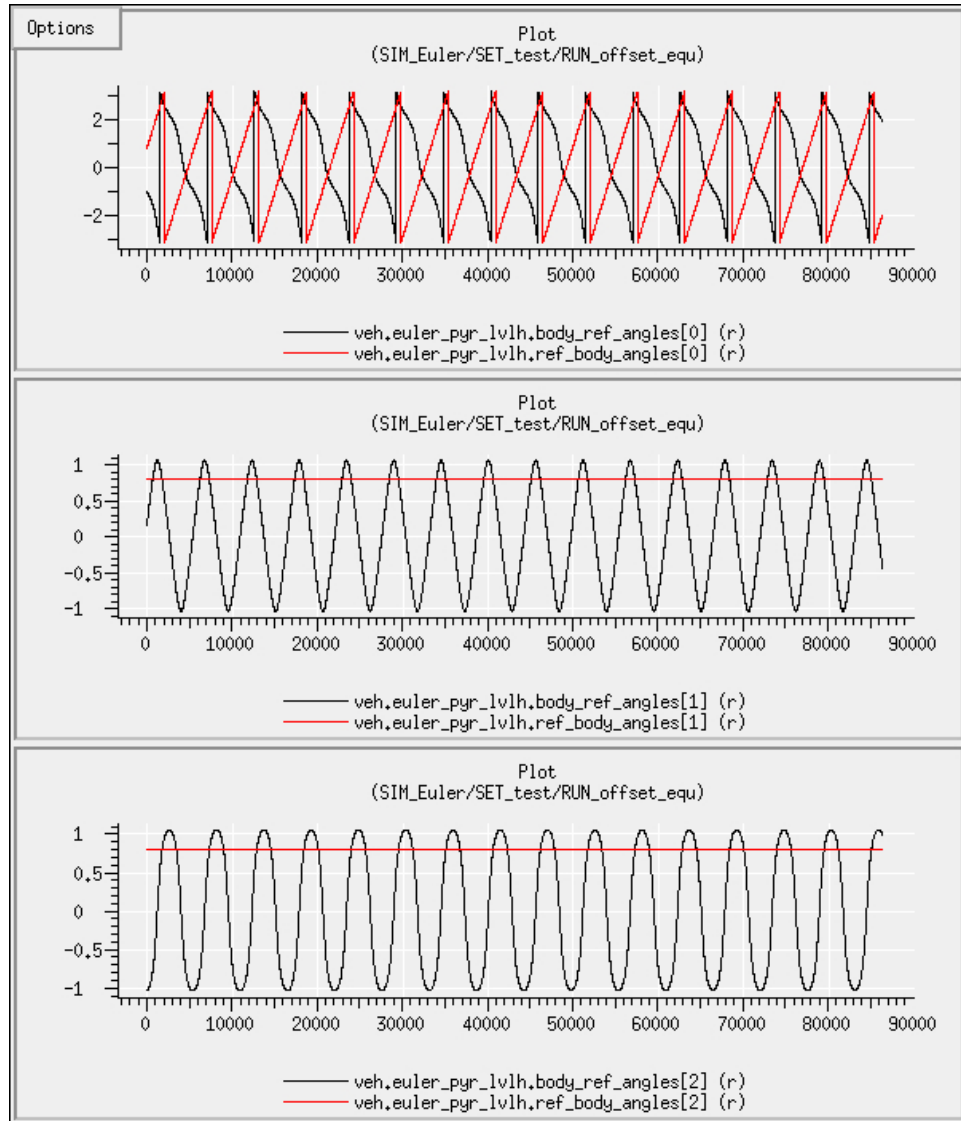
Figure 10.3: The Euler angles for the case in which the LVLH frame and body frame were initially un-aligned, and rotating with respect to each other on the pitch axis of the LVLH reference frame. Angles are expressed in a Pitch-Yaw-Roll sequence. Notice that when Pitch is first in the sequence, the angles associated with the transformation from the LVLH frame to the body frame (expressed in the LVLH frame) show a similar pattern to that in Figure 10.1, but that is not the case when representing the relative attitude from the body frame to the LVLH frame (this is expressed in the body frame).
