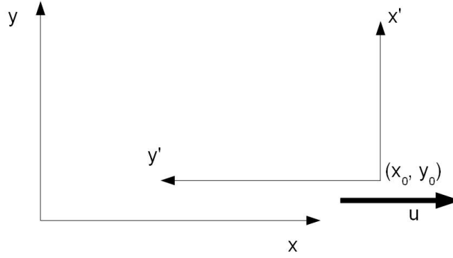
Figure 38.1: The momentary positions, velocity, and orientation of frames S and S'
