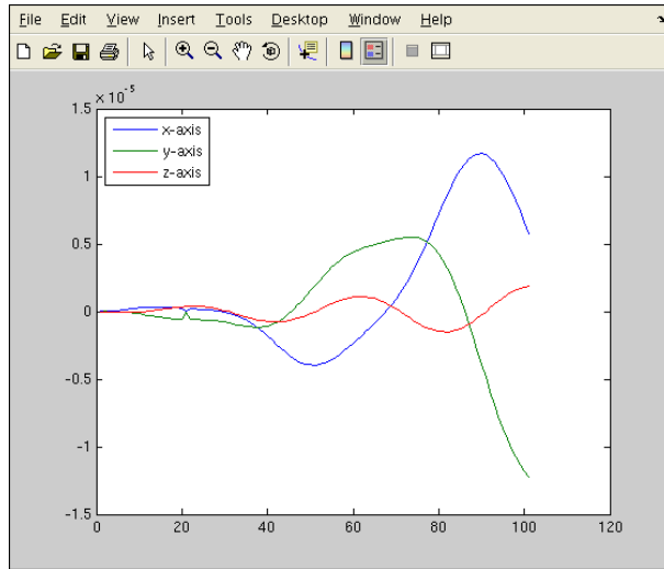
Figure 40.6: The variation with time of the difference between the analytical and numerical solutions for the position of A with respect to B.
