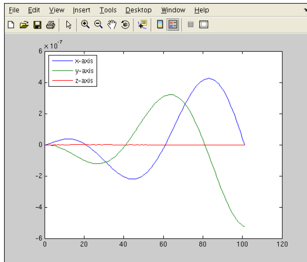
Figure 40.11: The variation with time of the difference between the analytical and numerical solutions for the angular velocity of B with respect to A.
