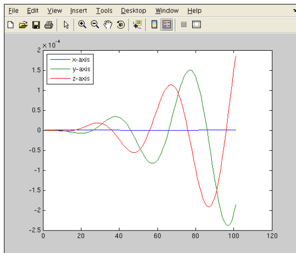
Figure 40.9: The variation with time of the difference between the analytical and numerical solutions for the position of B with respect to A.
