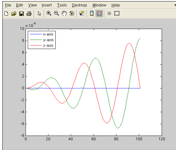
Figure 40.8: The variation with time of the difference between the analytical and numerical solutions for the angular velocity of A with respect to B.
