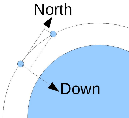
Figure 21.1: The effect of the curvature of an orbit on the relative state using rectilinear coordinates.
