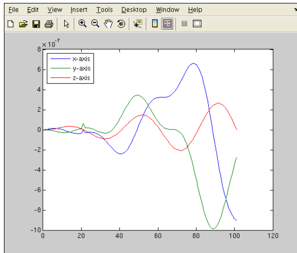
Figure 40.7: The variation with time of the difference between the analytical and numerical solutions for the velocity of A with respect to B.
