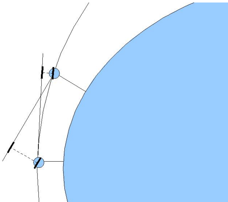
Figure 25.1: The effect of the difference between the curvature of an orbit and that of the reference ellipse on the relative state using rectilinear coordinates. The vehicle closer to the equator will exhibit a larger down component in its state than the vehicle farther from the equator.
