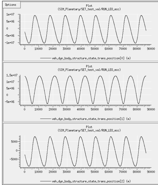
Figure 35.11: The variation of position with time, expressed in inertial coordinates.
