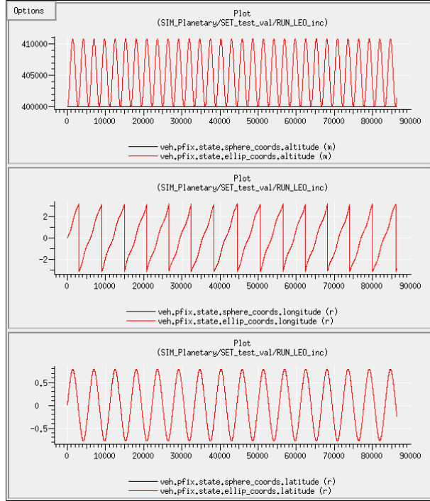
Figure 35.6: The variation of position with time, expressed in Altitude-Longitude-Latitude coordinates, both spherical and elliptical (geodetic).
