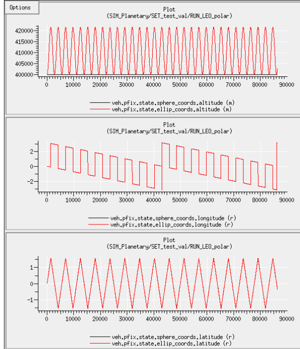
Figure 35.9: The variation of position with time, expressed in Altitude-Longitude-Latitude coordinates, both spherical and elliptical (geodetic).
