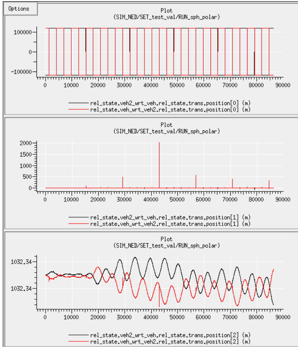
Figure 25.4: The relative states for a polar orbit, with spherical geometry used to define the reference frame.
