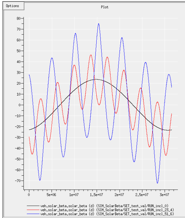
Figure 45.1: The variation of Solar Beta with time for the first three test cases. These are all circular orbits with orbital inclinations of 0, 23.4, and 51.6 degrees respectively
