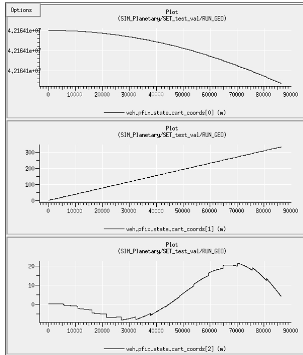
Figure 35.13: The variation of position with time, expressed in Cartesian coordinates.
