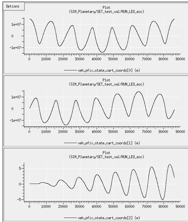
Figure 35.10: The variation of position with time, expressed in Cartesian coordinates.
