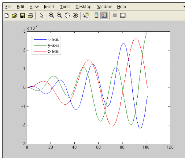
Figure 40.3: The variation with time of the difference between the analytical and numerical solutions for the velocity of A with respect to B.
