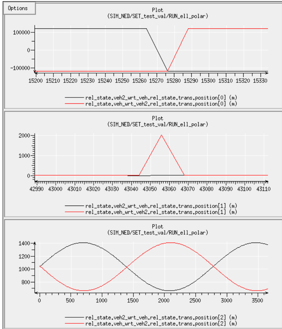
Figure 25.3: The relative states for a polar orbit, with elliptical geometry used to define the reference frame, zoomed in to locations of interest.
