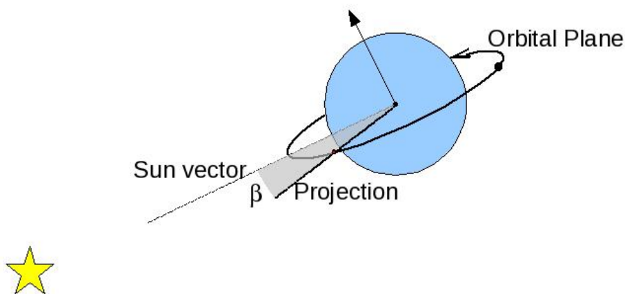
Figure 43.1: The definition of the Solar Beta angle. The arrow represents the orbital angular momentum vector. Note that the position of the vehicle (upper right) on the orbit is of no consequence to the determination of the Solar Beta angle.
