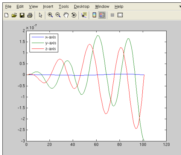
Figure 40.5: The variation with time of the difference between the analytical and numerical solutions for the velocity of B with respect to A.
