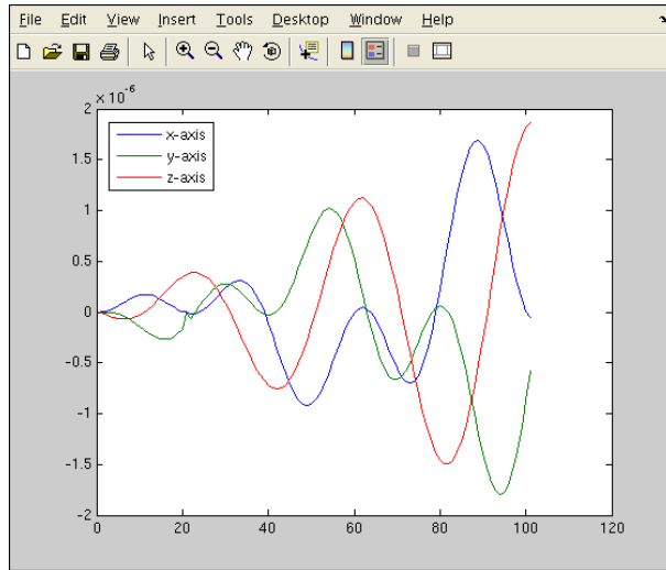
Figure 40.2: The variation with time of the difference between the analytical and numerical solutions for the position of A with respect to B.
