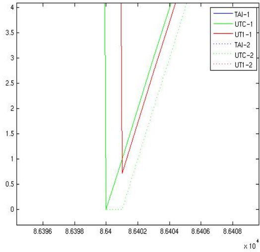
Figure 5.6: Values of UTC showing the addition of a leap second in the JEOD v5.4-compatible version, but not in previous versions.
