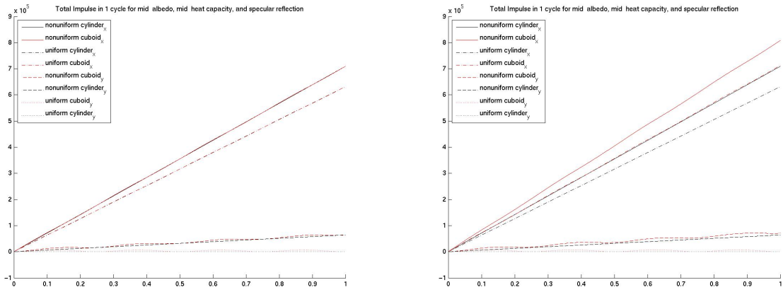
Figure 5.35: The data presented in the left graph is the center panel from figure 5.33, for which the cuboid surface area is equivalent to the cylinder surface area. The data presented in the second graph is the impulse when the cylinder is approximated as a cuboid while maintaining constant enclosed volume. For each graph, the x-axis represents time in cycles, and the y-axis represents accumulated impulse.
