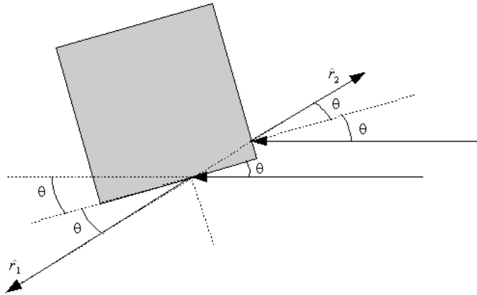
Figure 5.27: Schematic of the reflection from the two illuminated sides.
