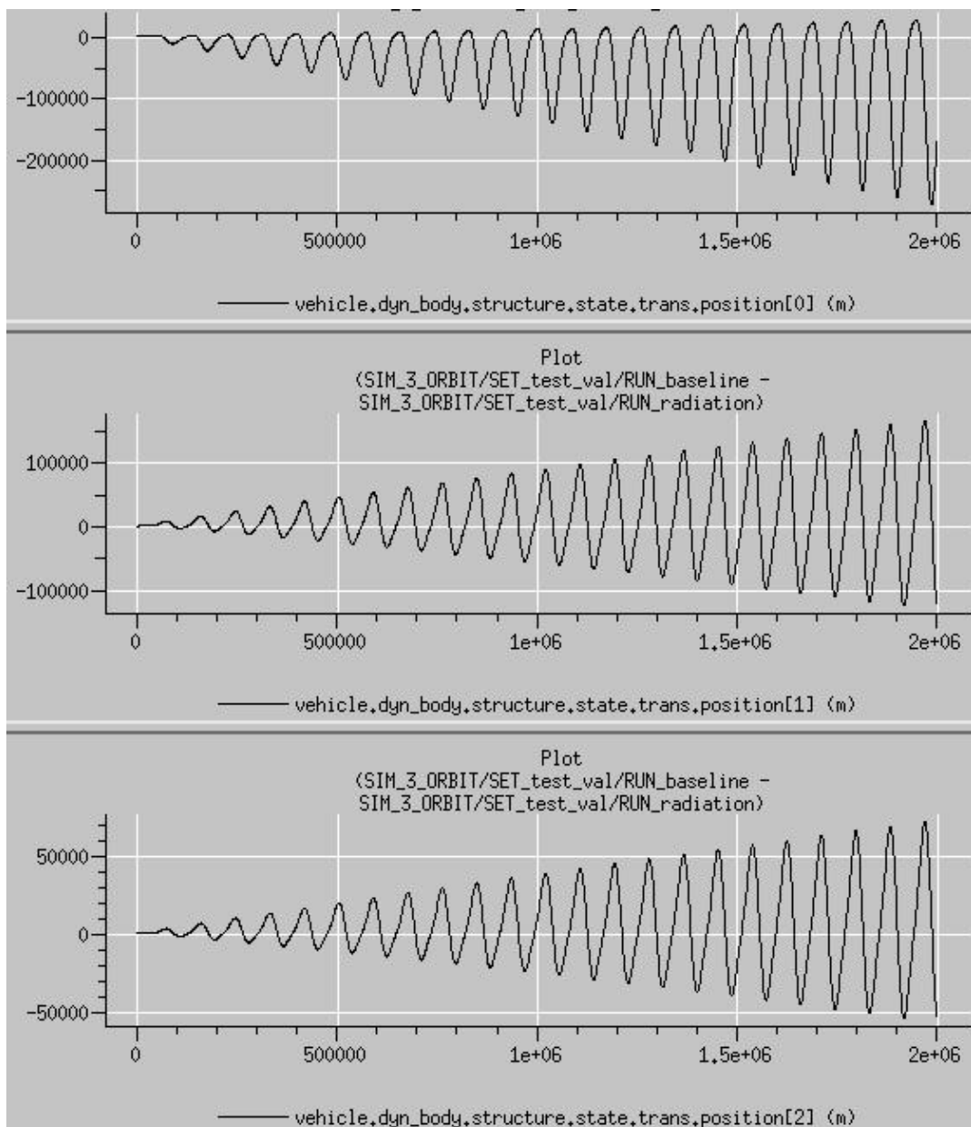
Figure 5.39: The effect on position of including the forces due to radiation pressure on an otherwise simple simulation of an Earth satellite at altitude comparable to that of a geosynchronous orbit.
