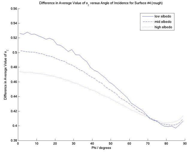
Figure 5.16: Differences between the analytic and numeric z-component of \langle \hat{s} \rangle for each of the 4 surface-profiles.
