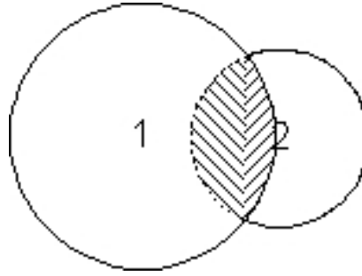
Figure 3.4: The area of the segment of a circle
