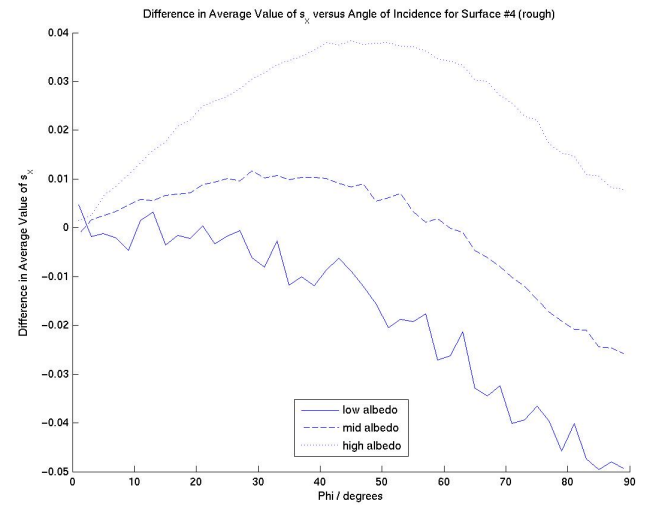
Figure 5.14: Differences between the analytic and numeric x-component of \langle \hat{s} \rangle for each of the 4 surface-profiles.
