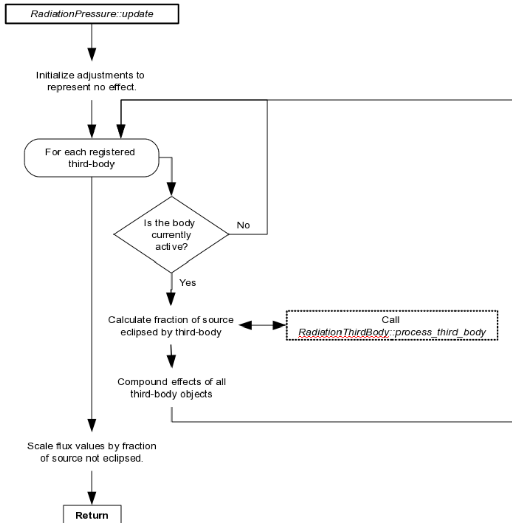
Figure 3.11: Flowcharts for Radiation Pressure Model (continued)
