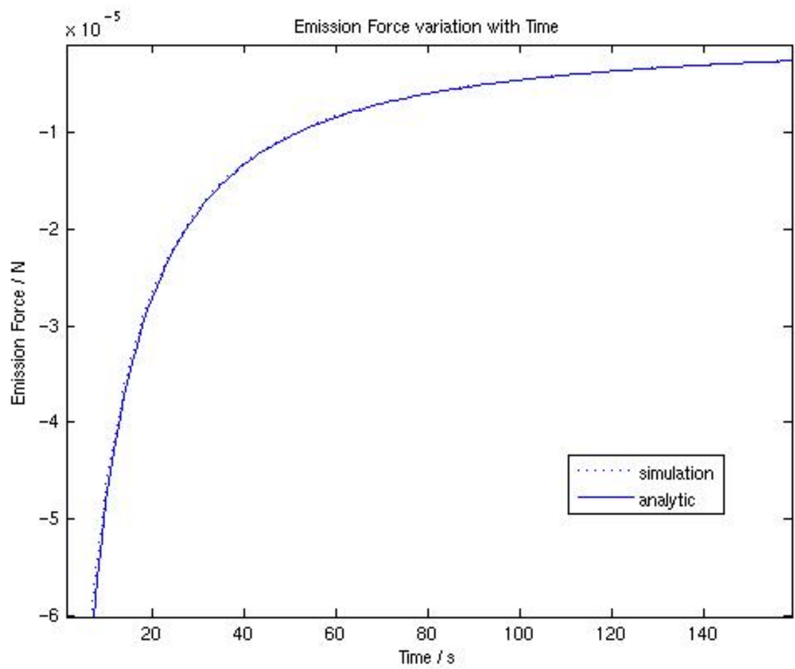
Figure 5.3: Variation with time of force, showing the simulation data and analytic solution overlaying.
