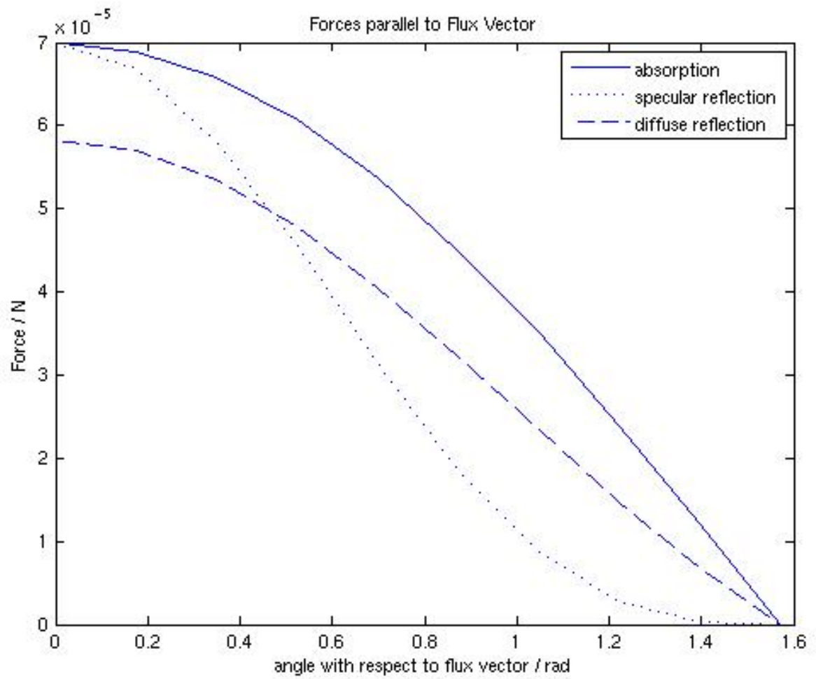
Figure 5.1: The components of the absorption, specular, and diffuse forces parallel to the flux vector as a function of the angle between the flux vector and the surface normal
