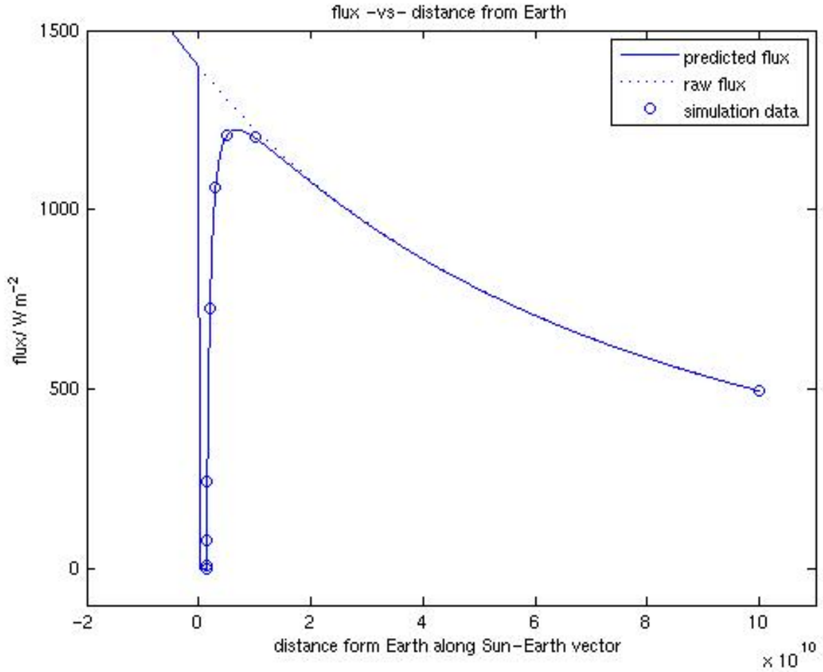
Figure 5.8: The flux of the vehicle as a function of distance from Earth on the Sun-Earth vector. The raw flux represents the solar flux without shadowing. The predicted flux represents the analytic function for flux with Earth shadowing included. Data points from the simulation are shown as circles.
