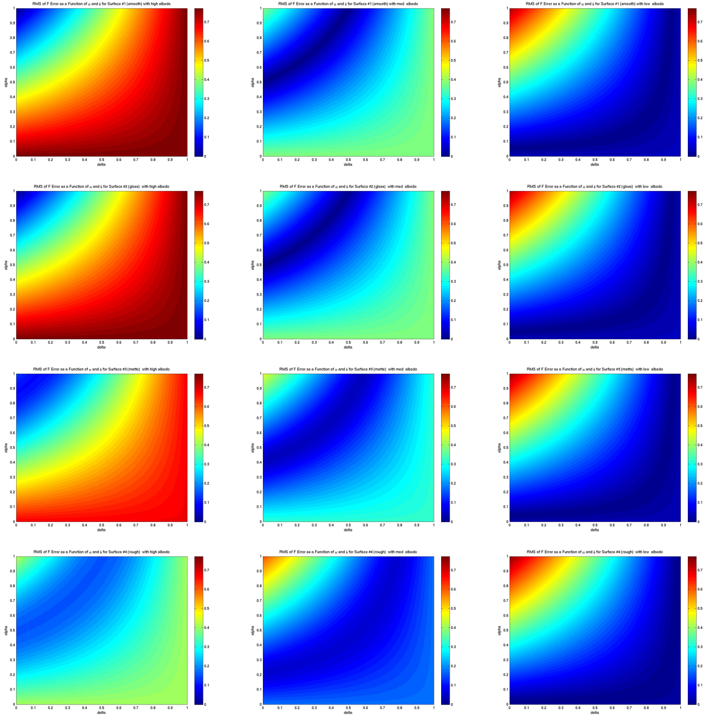
Figure 5.20: Differences in the value of the magnitude of the model force, comparing the numerical simulation to the simplified model, as a function of \alpha and \delta , presented in matrix formation with rows representing (from top) surface 1-4, and columns representing (from left) high to low albedo.
