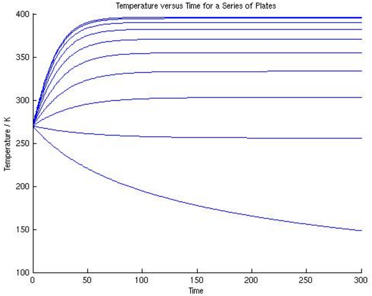
Figure 5.5: The variation of temperature with time over the 10 plates in the simulation.
