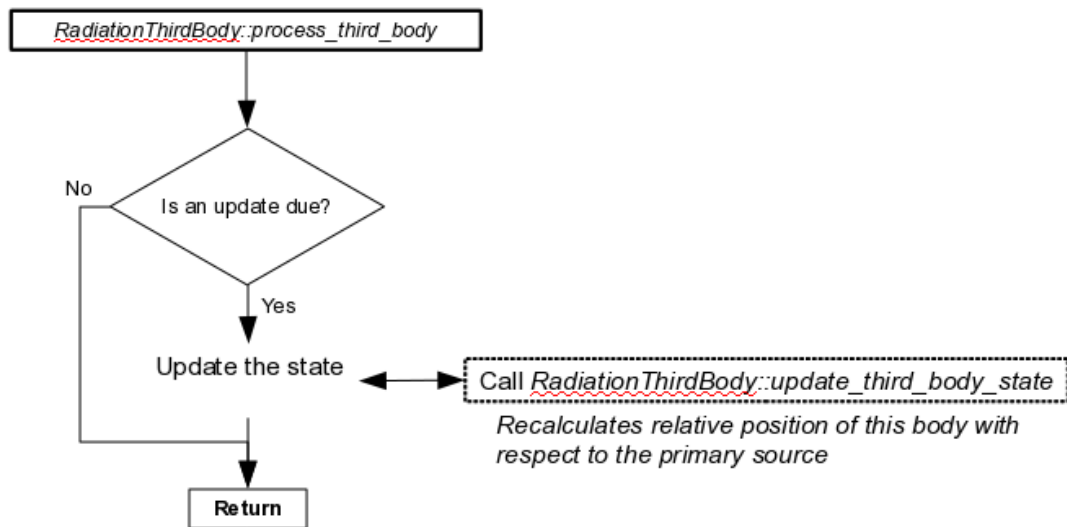
Figure 3.23: Flowchart for class RadiationThirdBody (continued)
