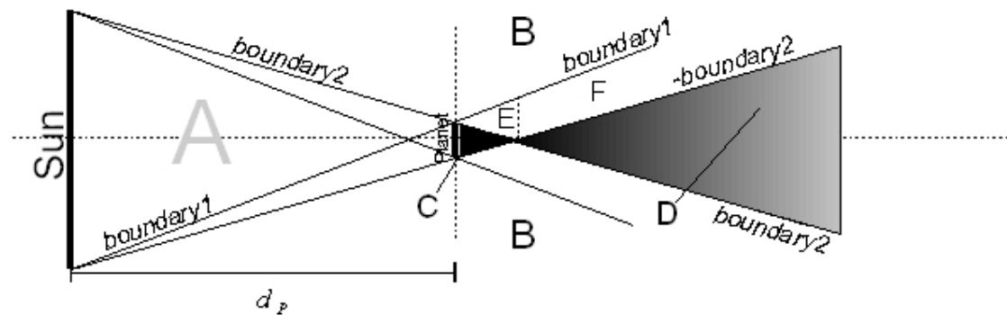
Figure 3.3: Conical shadow geometry
