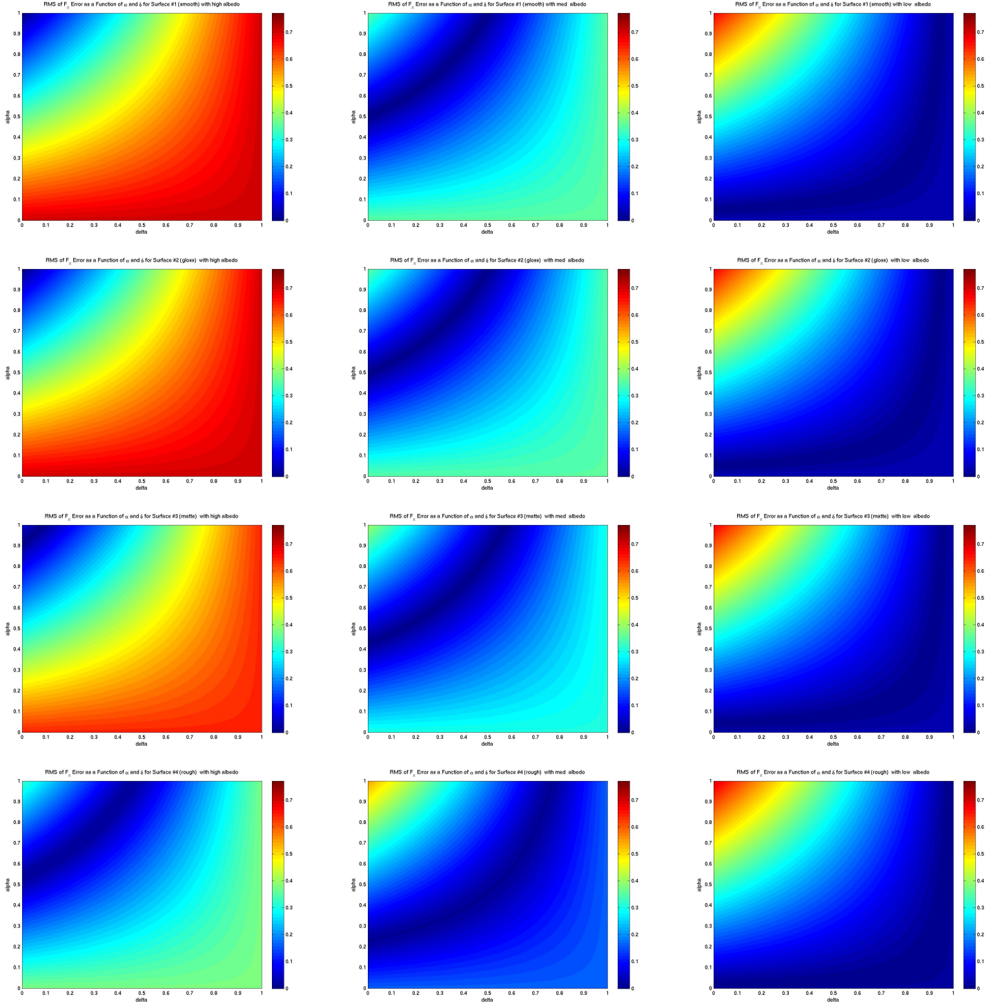
Figure 5.21: Differences in the value of the x-component of the model force, comparing the numerical simulation to the simplified model, as a function of \alpha and \delta , presented in matrix formation with rows representing (from top) surface 1-4, and columns representing (from left) high to low albedo.
