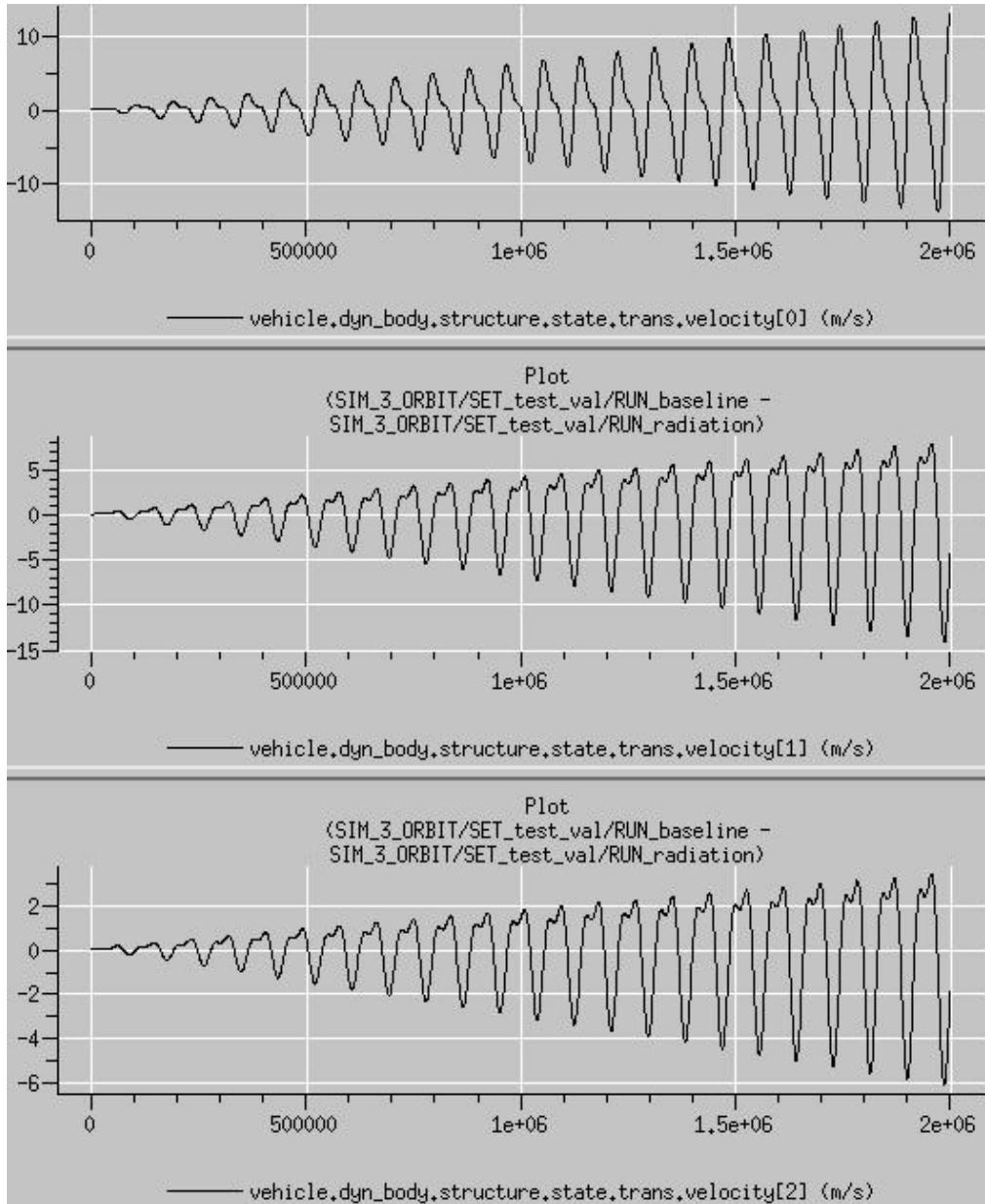
Figure 5.40: The effect on velocity of including the forces due to radiation pressure on an otherwise simple simulation of an Earth satellite at altitude comparable to that of a geosynchronous orbit.
