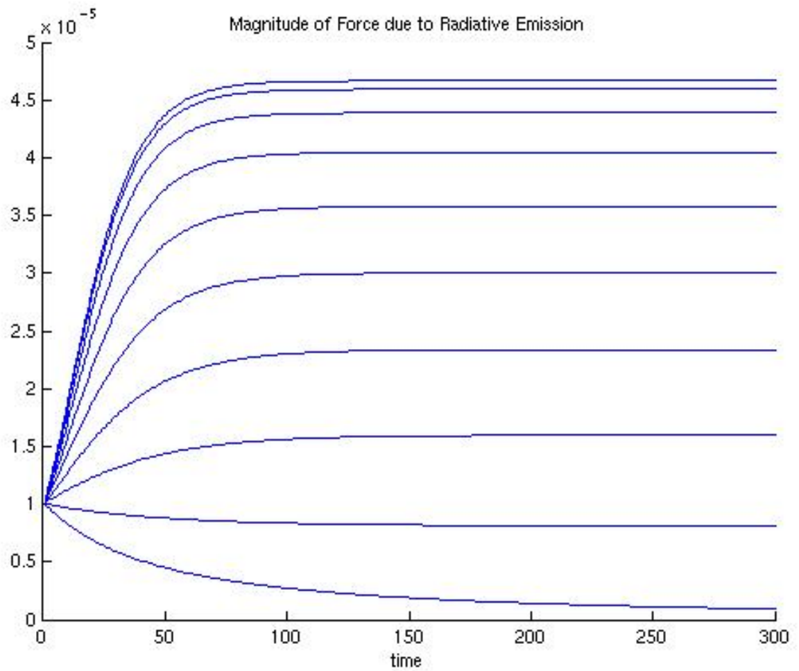
Figure 5.6: The variation with time of force, over the 10 plates in the simulation.
