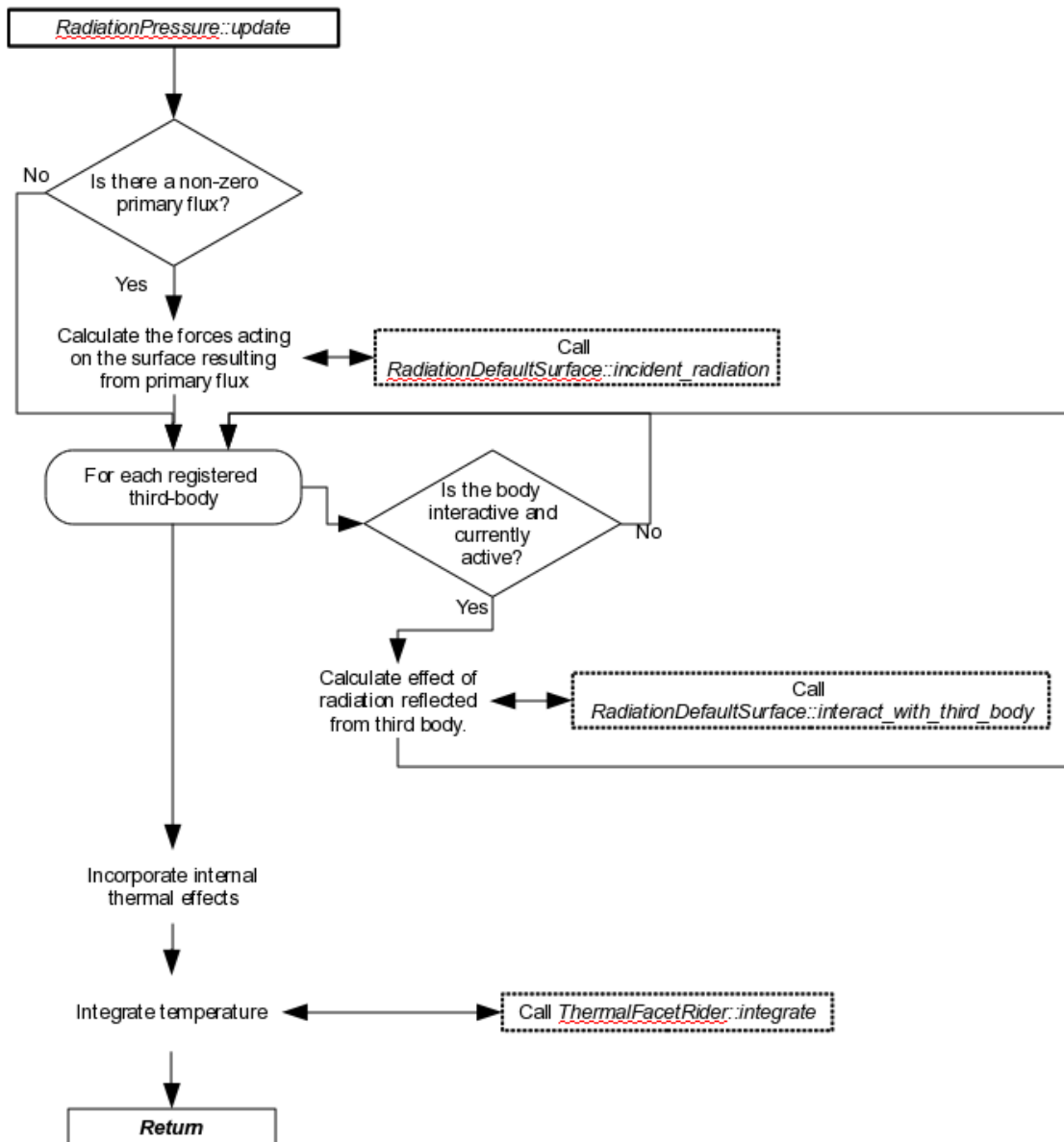
Figure 3.12: Flowcharts for class RadiationPressure (continued)
