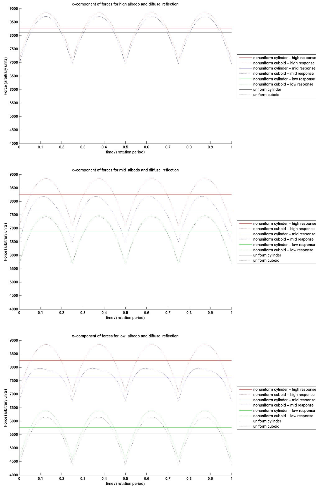
Figure 5.30: The x-component of force due to radiation with diffuse reflection. Each chart represents a different albedo, and contains plots for different temperature-response models. A model with low heat capacity will have a high temperature response.
