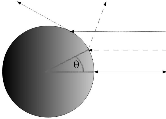
Figure 3.9: Light Rays Incident on a Specular Spherical Surface
