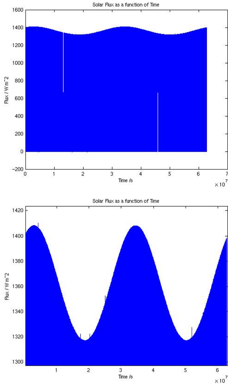
Figure 5.38: The long-term fluctuation in the solar flux observed by a satellite with period approximately 1 day. The upper graph gives an indication of the relative magnitude of the oscillation, while the lower graph gives a better indication of the absolute magnitude of the oscillation. The graph is solid because it also includes the daily oscillation between 0 and the background flux.
