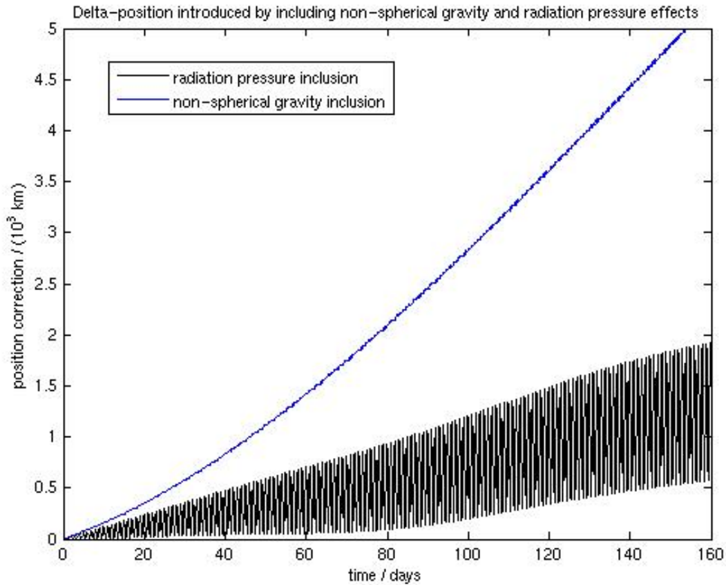
Figure 5.41: The result of including the effects of nonspherical gravity compared to the result of including the effects of radiation pressure, on an otherwise simple simulation of an Earth satellite at altitude comparable to that of a geosynchronous orbit.
