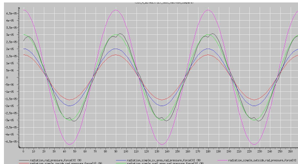
Figure 5.36: The x-component of the radiation forces for each of the surfaces; radiation.rad_pressure is the cubic surface; radiation.simple_inside fits inside the cube; radiation.simple_cx_area has the same cross-sectional area as the cube; radiation.simple_surf_area has the same surface area as the cube; radiation.simple_outside envelopes the cube.
