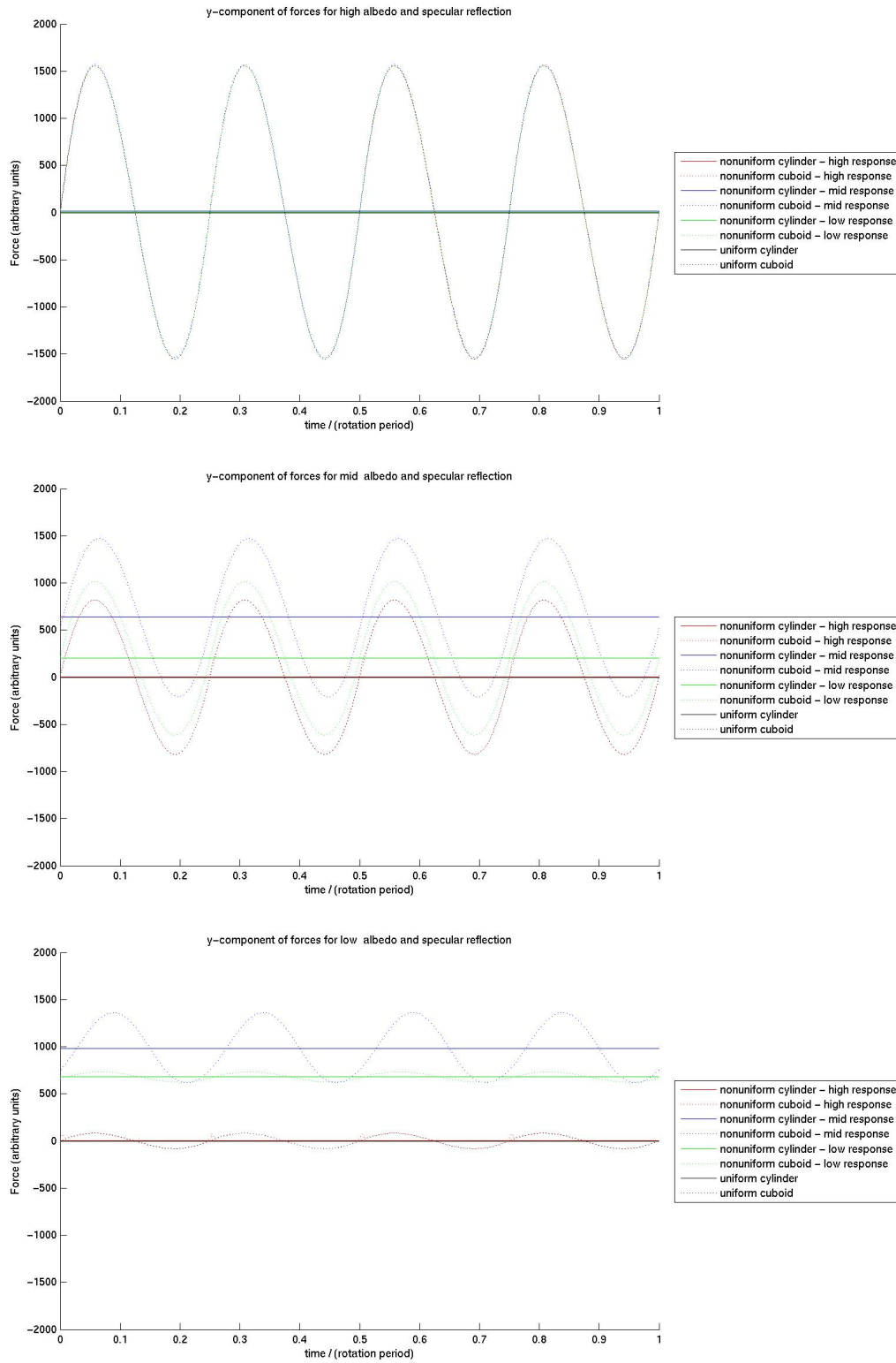
Figure 5.31: The y-component of force due to radiation with specular reflection. Each chart represents a different albedo, and contains plots for different temperature-response models. A model with low heat capacity will have a high temperature response.
