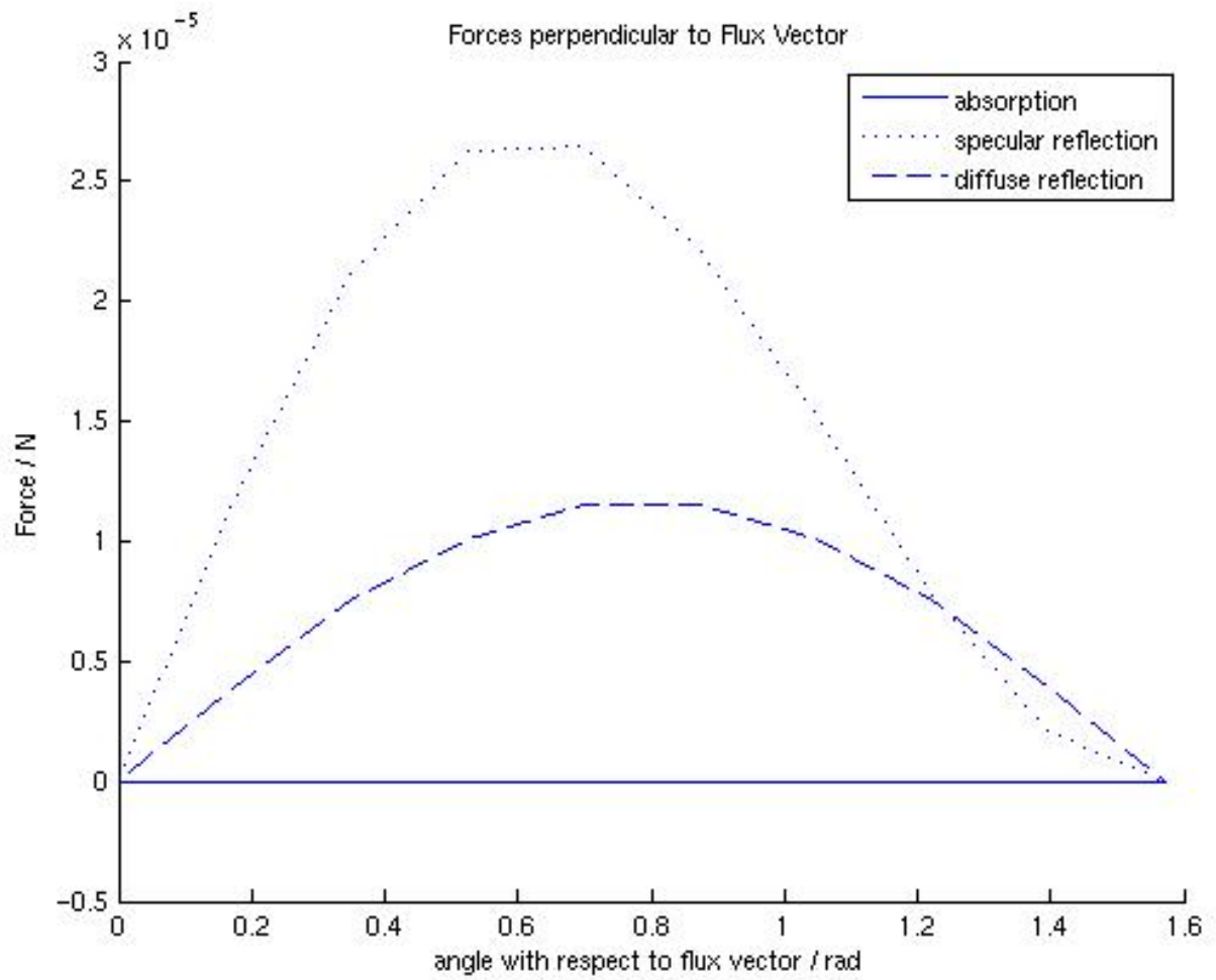
Figure 5.2: The components of the absorption, specular, and diffuse forces perpendicular to the flux vector as a function of the angle between the flux vector and the surface normal
