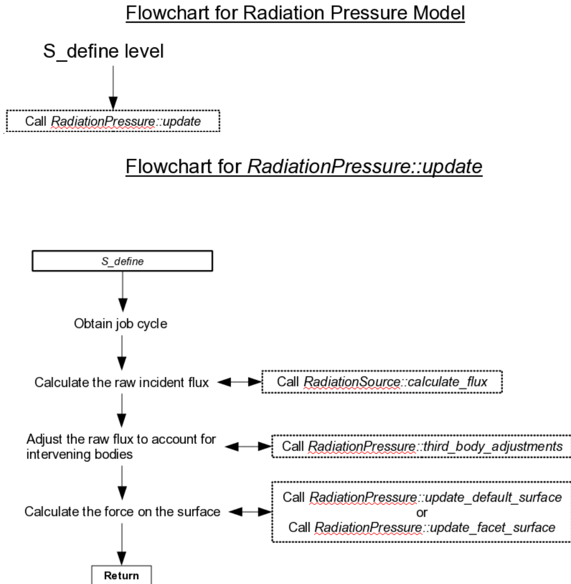
Figure 3.10: Flowcharts for Radiation Pressure Model
