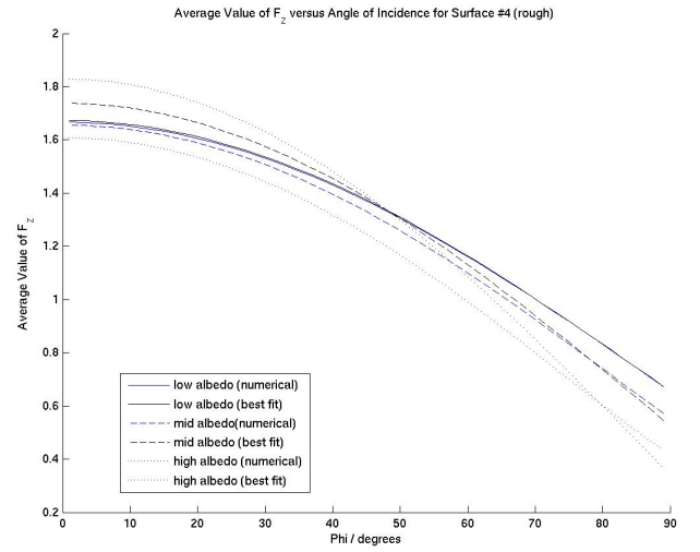
Figure 5.19: Mean values for the analytic and numeric z-component of the interaction force for each of the 4 surface-profiles.
