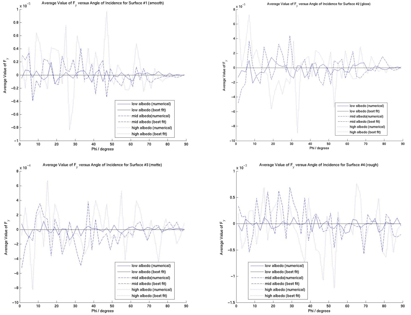
Figure 5.18: Mean values for the analytic and numeric y-component of the interaction force for each of the 4 surface-profiles.
