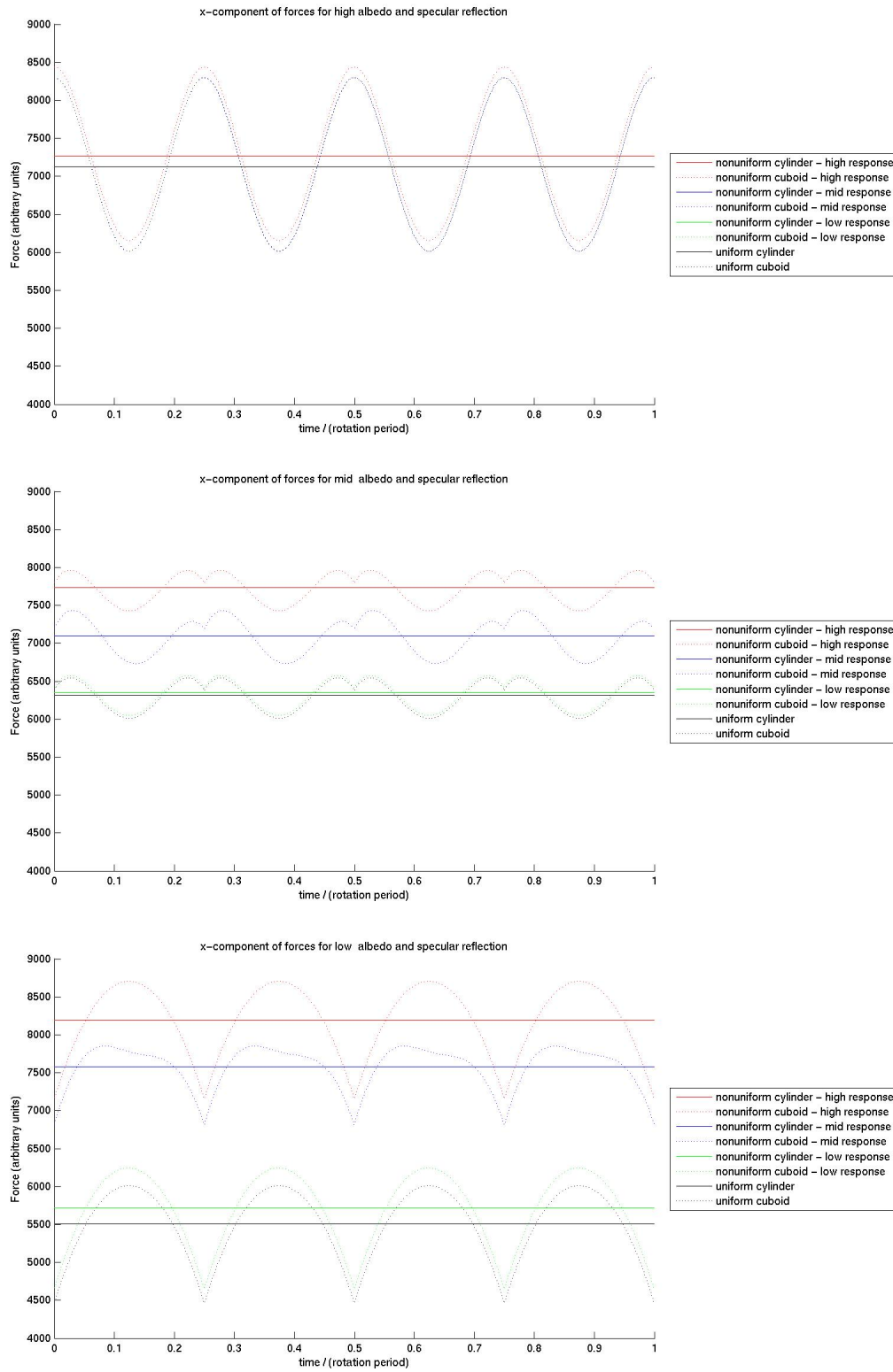
Figure 5.29: The x-component of force due to radiation with specular reflection. Each chart represents a different albedo, and contains plots for different temperature-response models. A model with low heat capacity will have a high temperature response.
