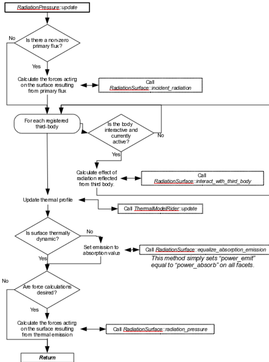
Figure 3.13: Flowcharts for class RadiationPressure (continued)
