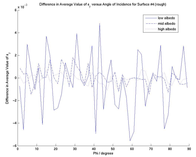
Figure 5.15: Differences between the analytic and numeric y-component of \langle \hat{s} \rangle for each of the 4 surface-profiles.
