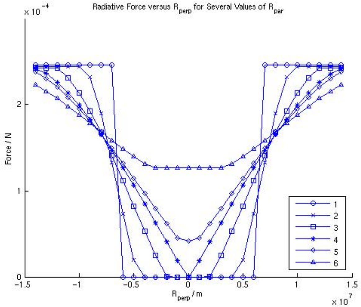
Figure 5.11: The magnitude of the radiative force as a function of r_{\text{perp}} for different values of r_{\text{par}}
