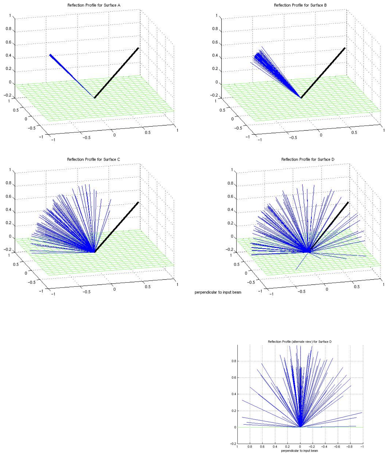
Figure 5.12: Reflection characteristics from four surfaces
