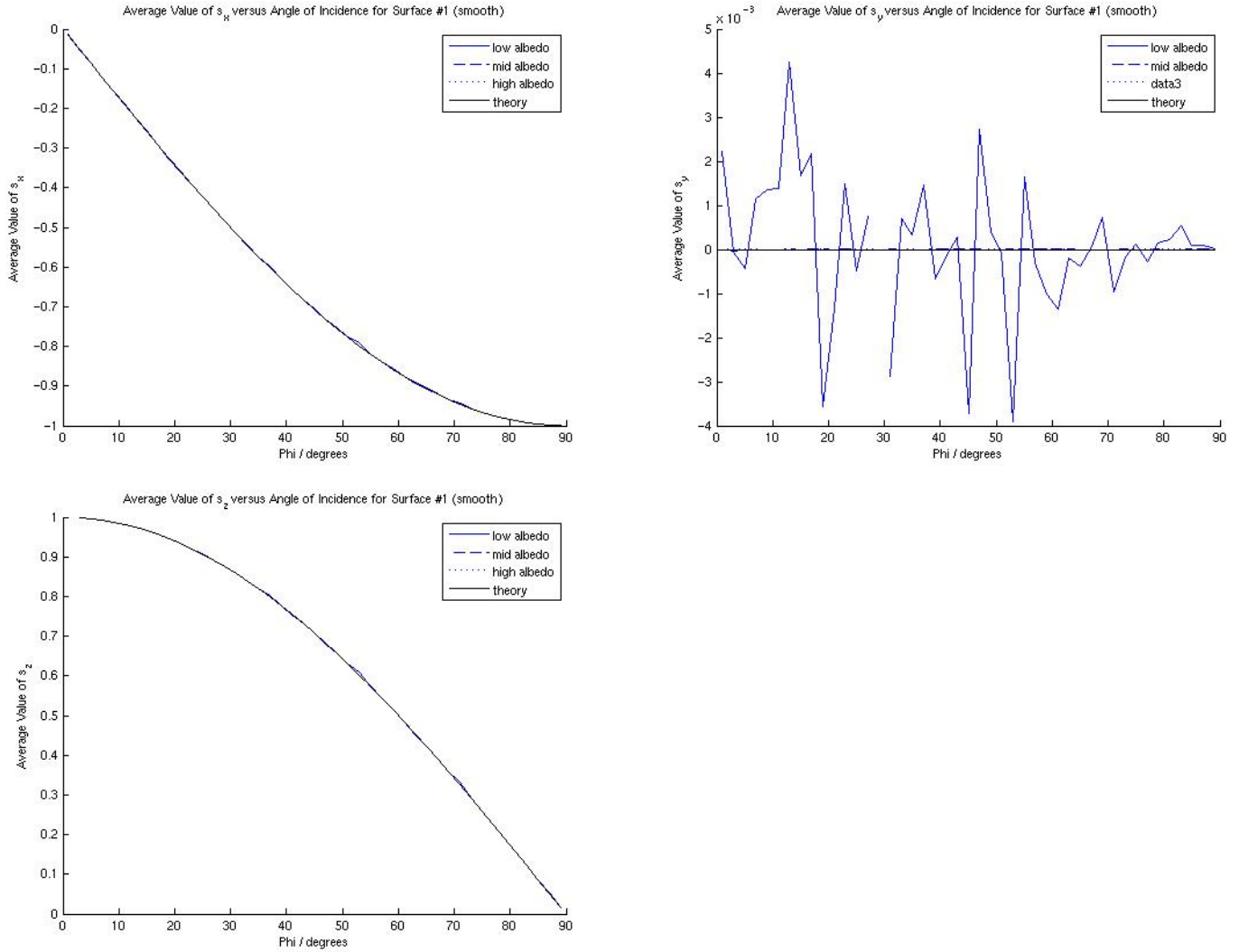
Figure 5.13: Analytical and numerical mean values for components of the reflection vector from a smooth surface as a function of incident angle
