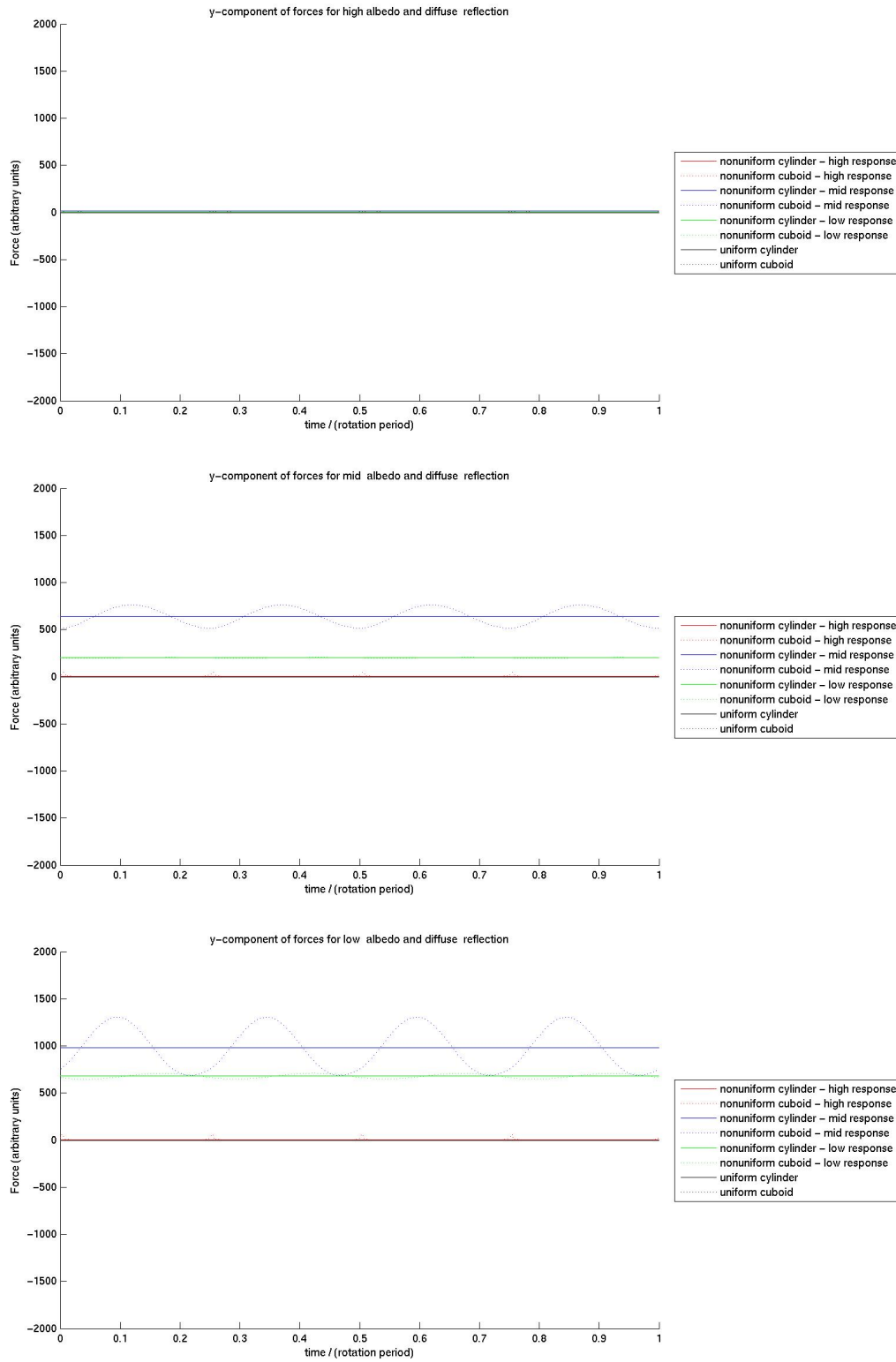
Figure 5.32: The y-component of force due to radiation with diffuse reflection. Each chart represents a different albedo, and contains plots for different temperature-response models. A model with low heat capacity will have a high temperature response.
