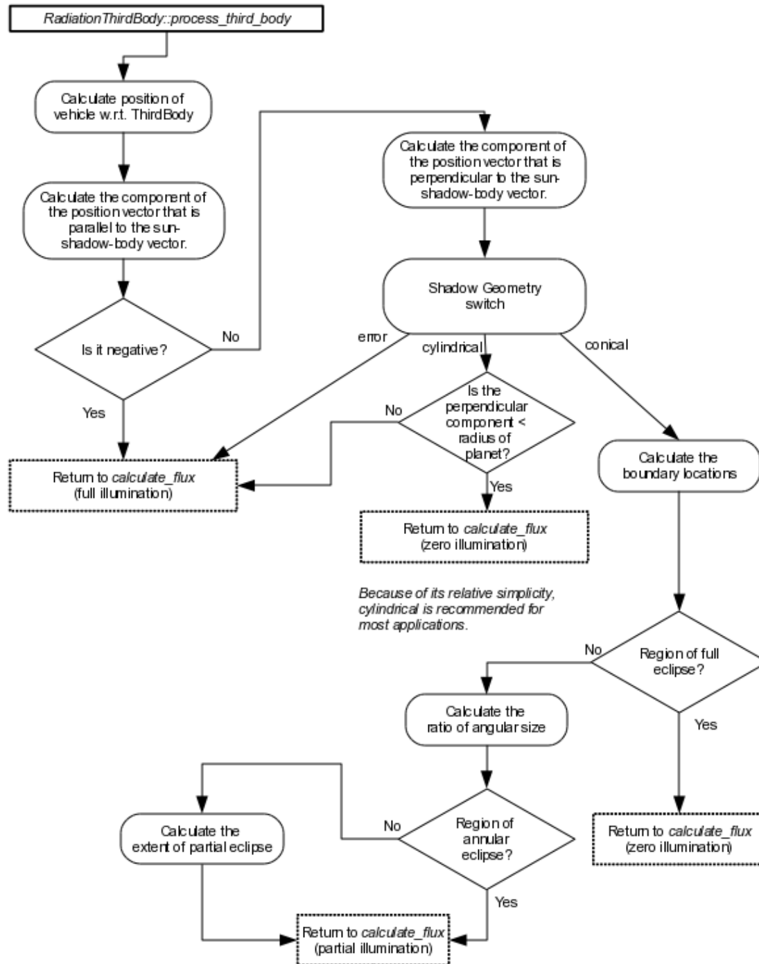
Figure 3.22: Flowchart for class RadiationThirdBody
