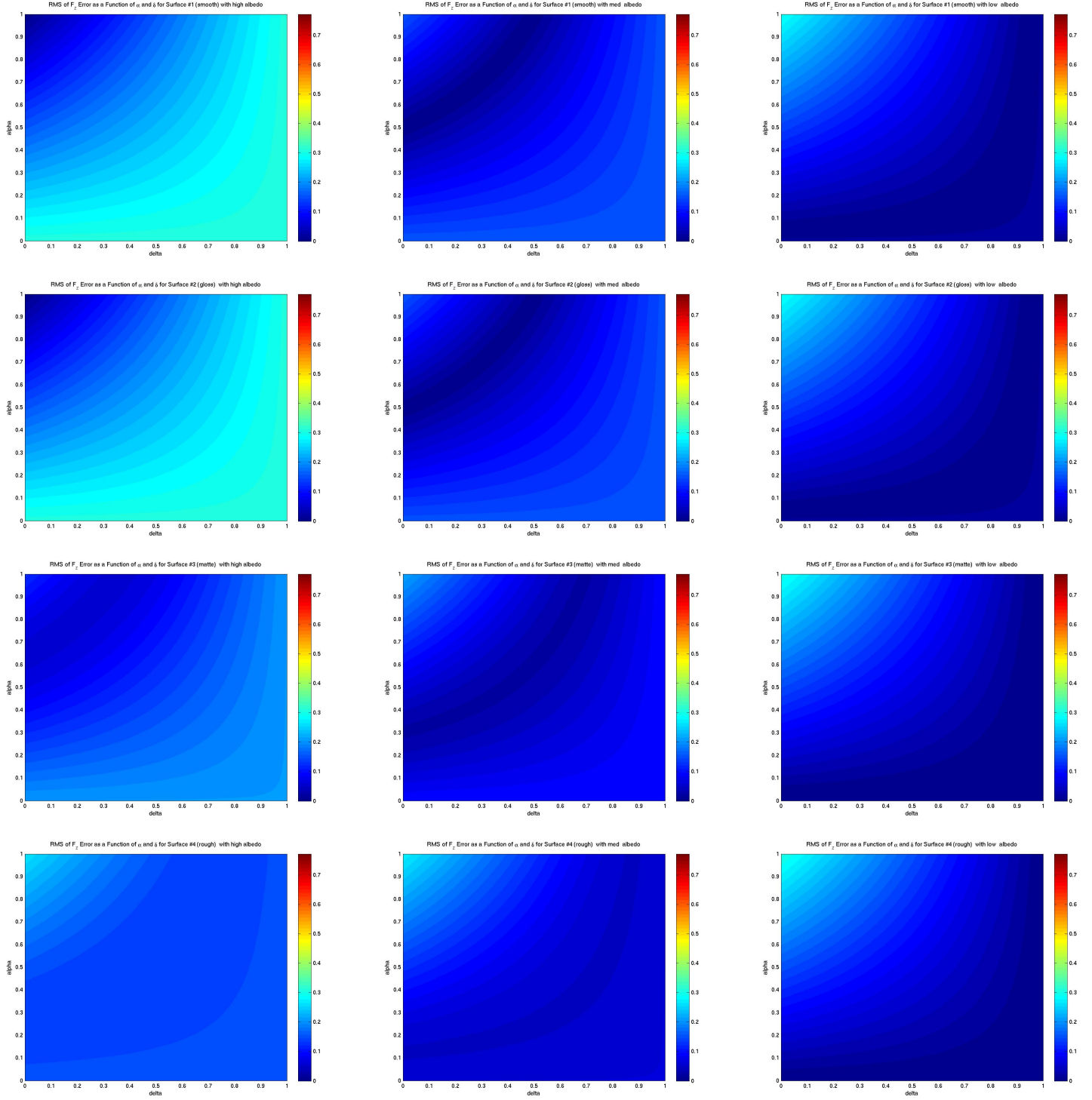
Figure 5.22: Differences in the value of the z-component of the model force, comparing the numerical simulation to the simplified model, as a function of \alpha and \delta , presented in matrix formation with rows representing (from top) surface 1-4, and columns representing (from left) high to low albedo.
