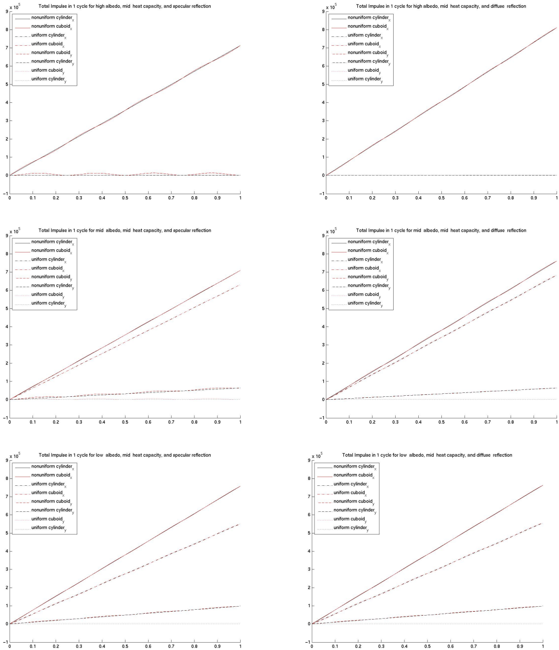
Figure 5.34: The data in the left column is a copy of the center column from figure 5.33, with specular reflection. The data in the right-column is from similar runs but with diffuse reflection. For each graph, the x-axis represents time in cycles, and the y-axis represents accumulated impulse.
