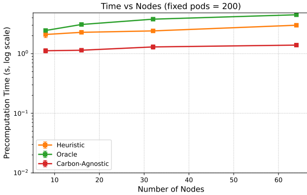
Fig. 7. Median precompute runtime versus node count at fixed 200 pods (overlay across algorithms; error bars where available denote \pm 1\sigma ).
