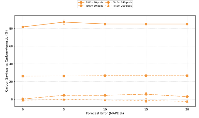
Fig. 10. Carbon savings relative to the carbon-agnostic baseline when schedulers consume noisy forecasts with various MAPE levels. Thin lines show TotEm savings for four representative pod counts. Decisions use the noisy traces; scoring uses the original Electricity Maps trace.
