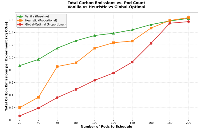
Fig. 4. Total carbon emissions vs. pod count ( coverage-inclusive ). Emissions are computed using a shared model (operational + amortized embodied). Inclusive results reflect each algorithm's actual coverage at a given scale.
