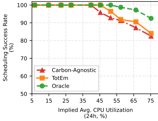
Fig. 4. Scheduling success rate vs. implied average cluster CPU utilization over 24 hours. Higher is better. Used jointly with inclusive emissions to disambiguate feasibility from carbon efficiency.
