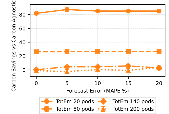
Fig. 7. Carbon savings relative to the carbon-agnostic baseline when schedulers consume noisy forecasts with various MAPE levels. Thin lines show TotEm savings for four representative pod counts. Decisions use the noisy traces; scoring uses the original Electricity Maps trace.
