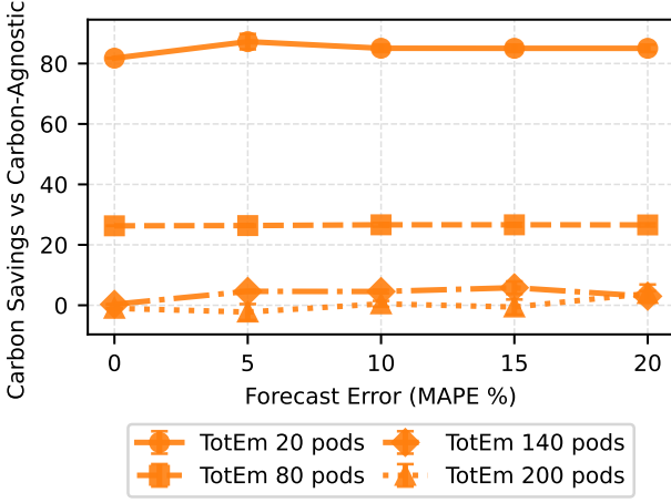
Fig. 10. Carbon savings relative to the carbon-agnostic baseline when schedulers consume noisy forecasts with various MAPE levels. Thin lines show TotEm savings for four representative pod counts. Decisions use the noisy traces; scoring uses the original Electricity Maps trace.
