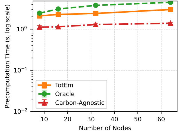
Fig. 7. Median precompute runtime versus node count at fixed 200 pods (overlay across algorithms; error bars where available denote \pm 1\sigma ).
