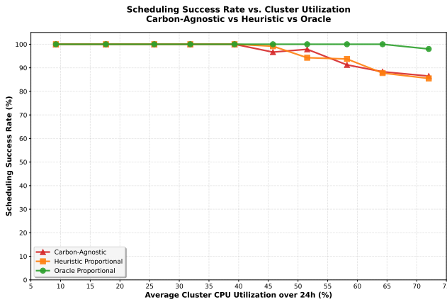
Fig. 7. Scheduling success rate vs. implied average cluster CPU utilization over 24 hours. Higher is better. Used jointly with inclusive emissions to disambiguate feasibility from carbon efficiency.
