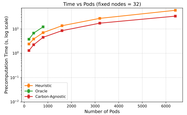
Fig. 9. Median precompute runtime versus pod count at fixed 32 nodes (overlay across algorithms; error bars where available denote \pm 1\sigma ).
