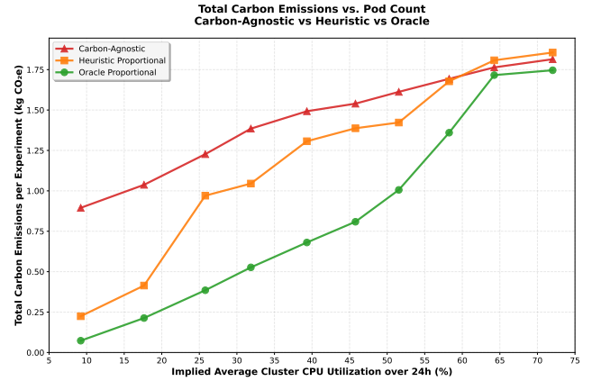
Fig. 5. Total carbon emissions vs. implied average cluster CPU utilization over 24 hours (coverage-inclusive). Emissions are computed using a shared model (operational + amortized embodied). Inclusive results reflect each algorithm's actual coverage at a given workload intensity.
