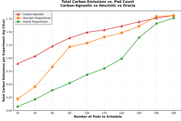
Fig. 5. Total carbon emissions vs. pod count ( coverage-inclusive ). Emissions are computed using a shared model (operational + amortized embodied). Inclusive results reflect each algorithm's actual coverage at a given scale.
