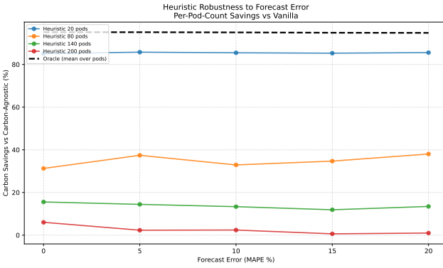
Fig. 10. Carbon savings relative to the carbon-agnostic baseline when schedulers consume noisy forecasts with various MAPE levels. Thin lines show heuristic savings for four representative pod counts; the dashed line shows the Oracle (MILP) upper bound averaged over pod counts. Decisions use the noisy traces; scoring uses the original Electricity Maps trace.
