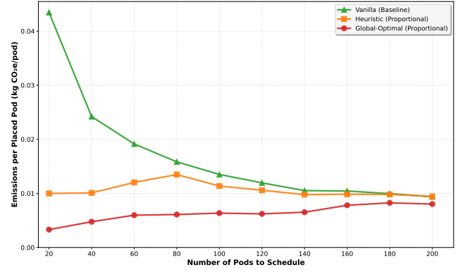
Emissions per Pod vs. Pod Count Vanilla vs Heuristic vs Global-Optimal
