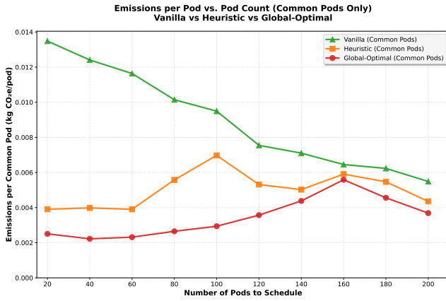
Fig. 6. Emissions per common pod (kg CO 2 e/pod) vs. pod count. Lower values indicate higher placement quality for identical work.
