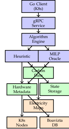
Fig. 1. Carbon-aware orchestration system architecture with component interactions and data flow.
