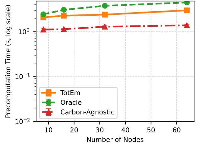
Fig. 7. Median precompute runtime versus node count at fixed 200 pods (overlay across algorithms; error bars where available denote \pm 1\sigma ).
