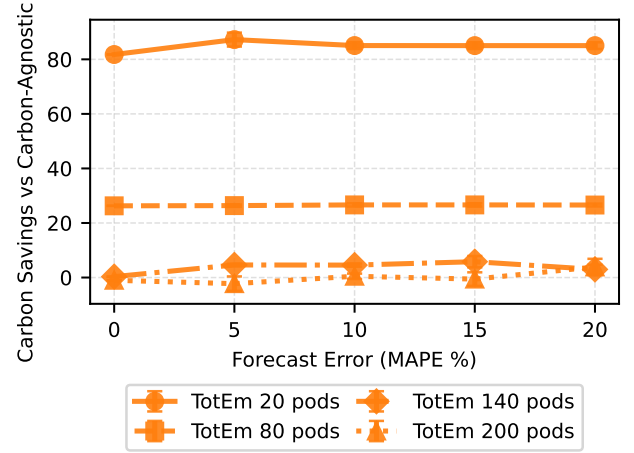
Fig. 10. Carbon savings relative to the carbon-agnostic baseline when schedulers consume noisy forecasts with various MAPE levels. Thin lines show TotEm savings for four representative pod counts. Decisions use the noisy traces; scoring uses the original Electricity Maps trace.
