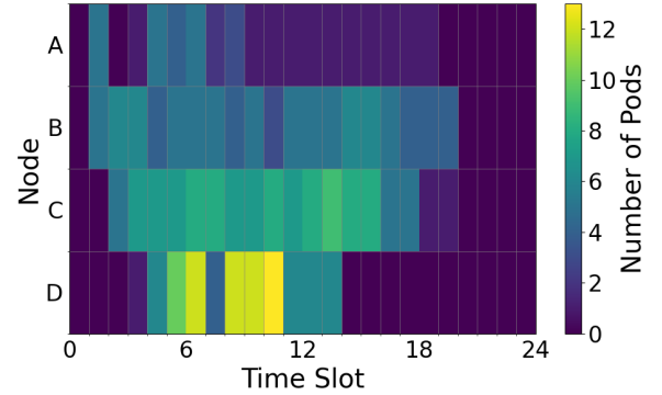
Fig. 3. TotEm (operational+embodied) scheduling. Incorporating amortized embodied costs drives the scheduler to pack pods denser, ensuring that the manufacturing carbon “investment” of each active node is fully utilized.
