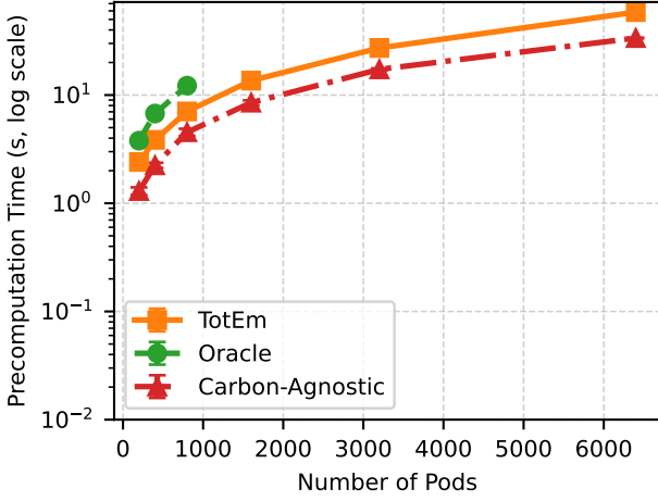
Fig. 8. Median precompute runtime versus pod count at fixed 32 nodes (overlay across algorithms; error bars where available denote \pm 1\sigma ).
