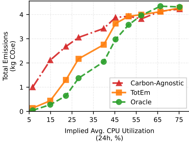
Fig. 4. Total carbon emissions vs. implied average cluster CPU utilization over 24 hours (coverage-inclusive). Emissions are computed using a shared model (operational + amortized embodied). Inclusive results reflect each algorithm's actual coverage at a given workload intensity.
