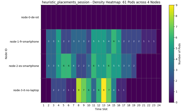
Fig. 1. Scheduling decisions using operational emissions only. The algorithm optimizes placement based solely on electricity carbon intensity, leading to concentrated utilization patterns that may overlook hardware embodied carbon implications.
