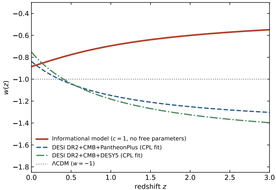
Equation of state
