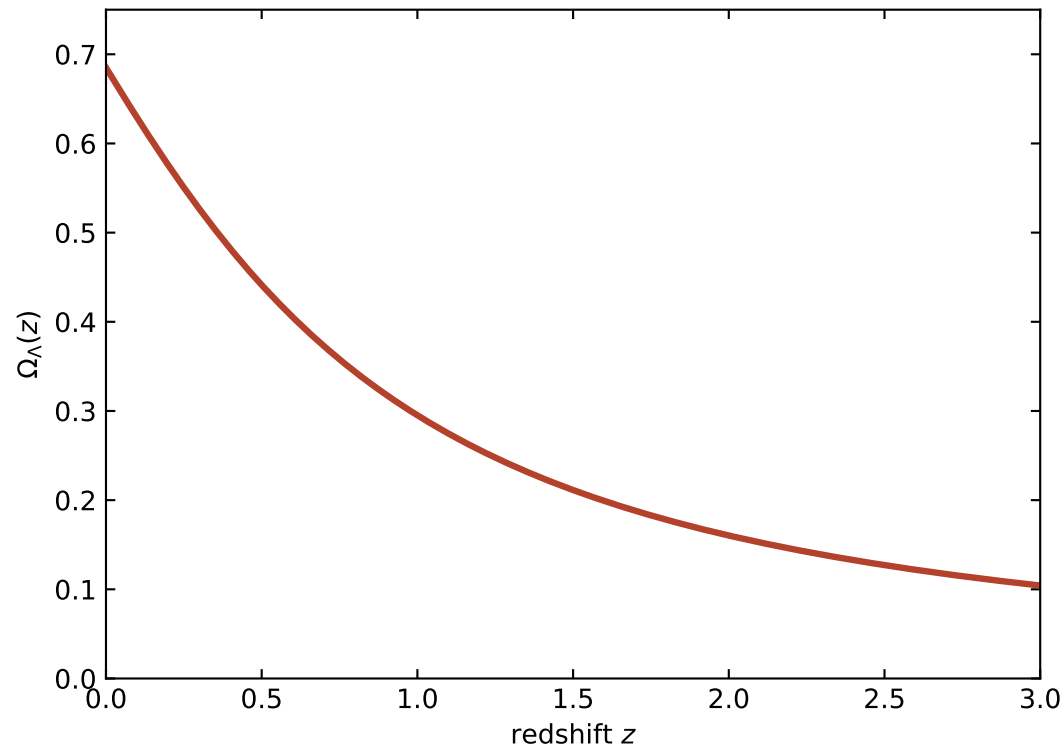
Dark-energy fraction \Omega_\Lambda(z)
