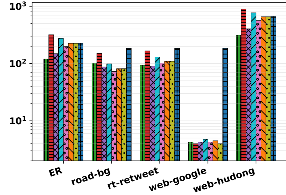
(c) kcore
