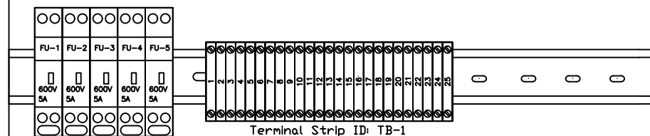
Wireway: Middle Section
