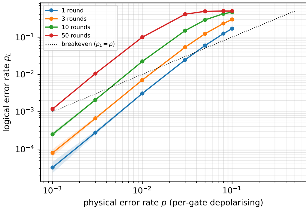
Rep-3 [[3,1,2]] , circuit-level noise, Stim + PyMatching MWPM 10^6 shots/point, software-only (not this project's own decoder)
