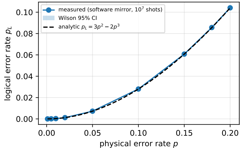
Rep-3 [[3,1,2]] , IID bit-flip
