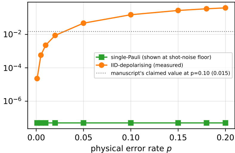
Shor [[9,1,3]]
