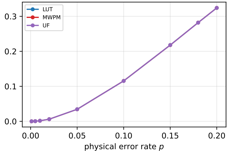
Steane [[7,1,3]] , IID-depolarising (3 decoder modes, real z-test in caption)
