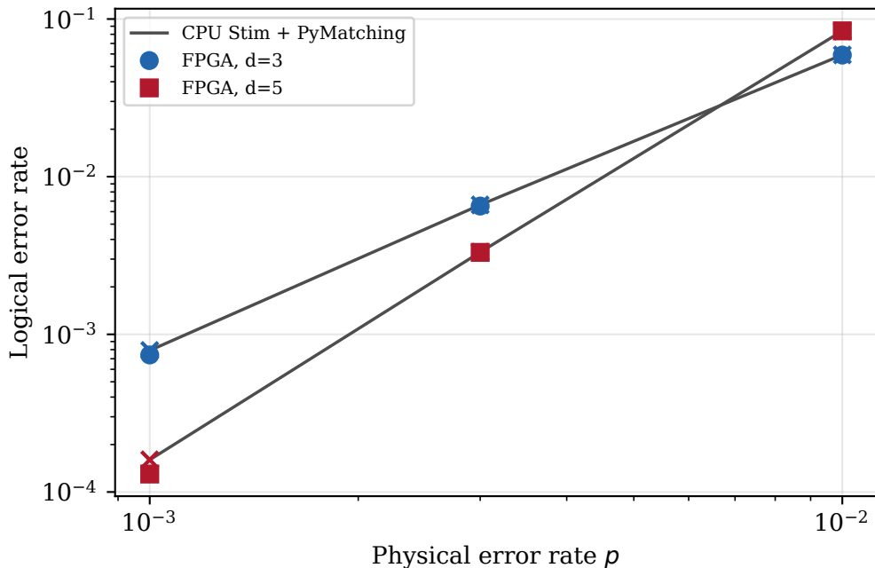
Tier 5: logical error rate, FPGA syndromes vs. CPU Stim (surface code, rotated memory Z, 10^6 shots/point)
