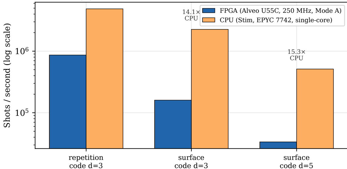
Mode A throughput: FPGA vs. single-core CPU Stim (SHOTS=64/launch)
