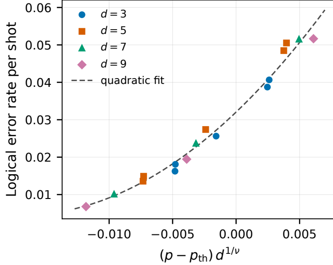
Fig. 2 Finite-size-scaling collapse of the baseline data onto a single quadratic. Provenance: T4
