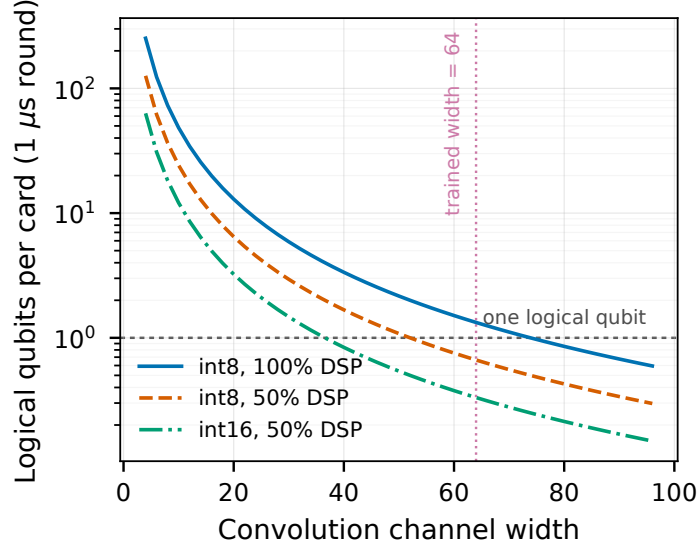
Fig. 3 Sustainable logical qubits per card versus convolution width, from the compute roofline. Provenance: T4 bound from T1 device counts
