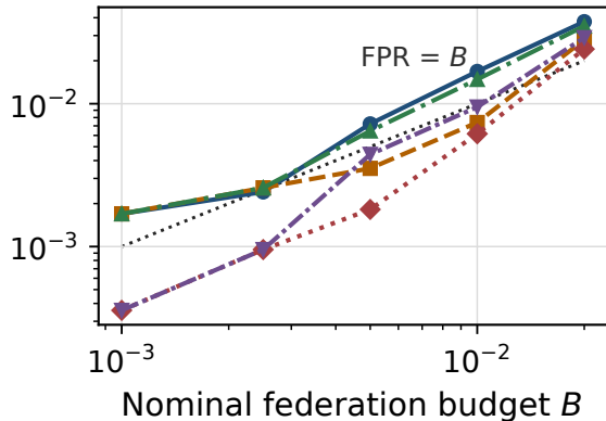
(a) Nominal versus realized FPR
