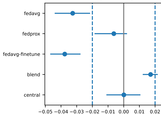
known-family-recall-change
