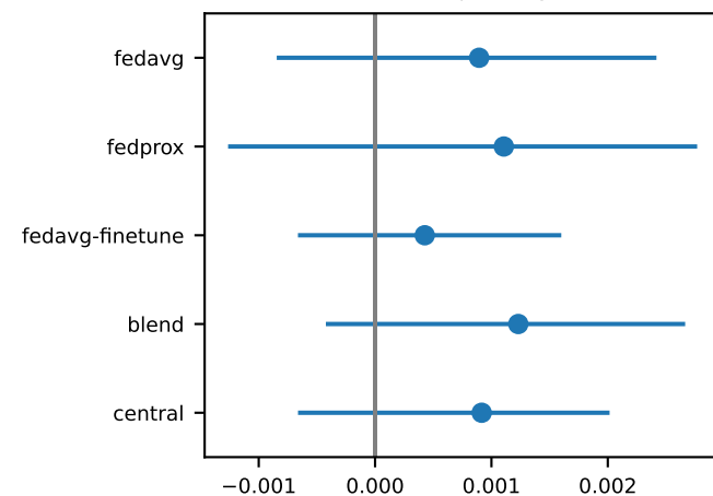
realised-fpr-change
