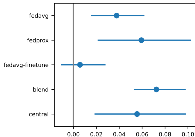
own-domain-unseen-recall-change
