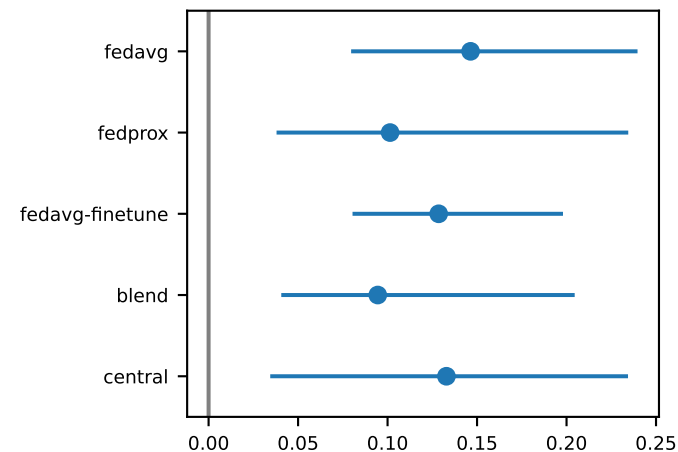
worst-client-unseen-recall-change
