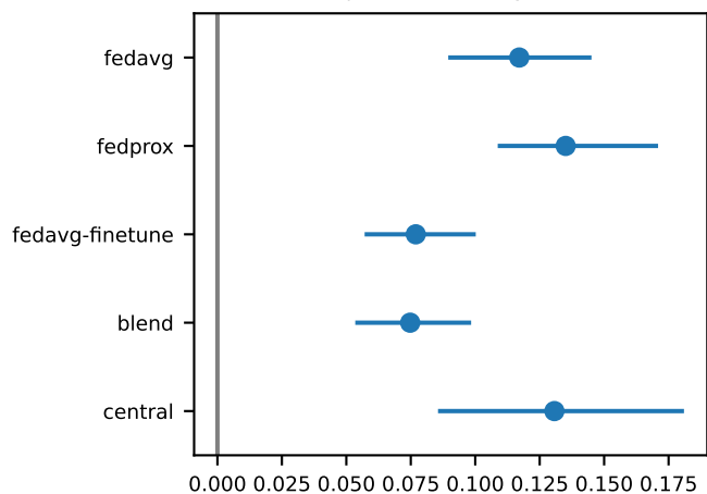
paired-seed-ctk-gain
