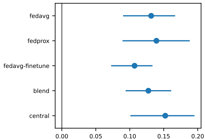
federation-unseen-recall-change
