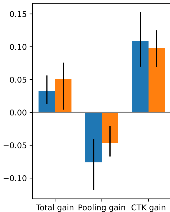
own-domain-unseen-recall
