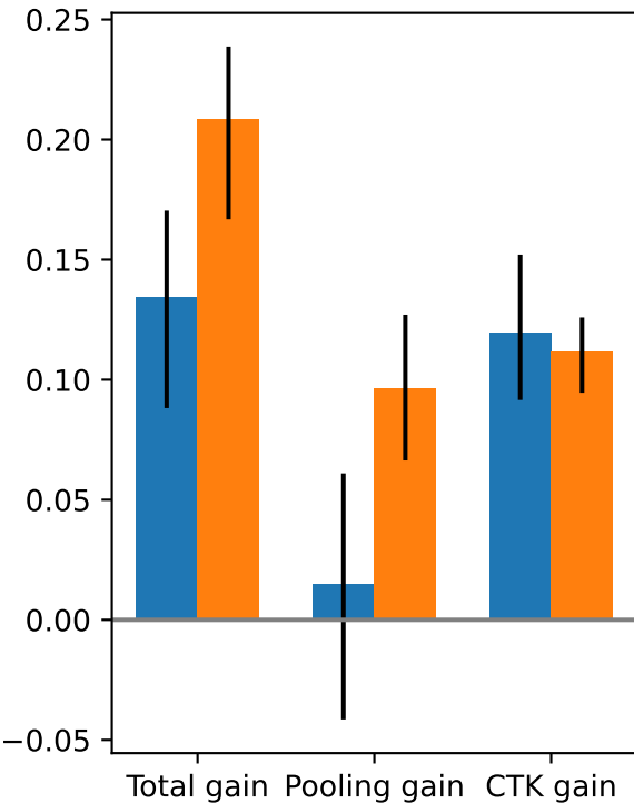
federation-unseen-recall
