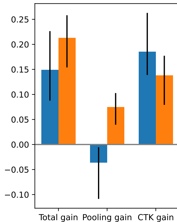
worst-client-unseen-recall
