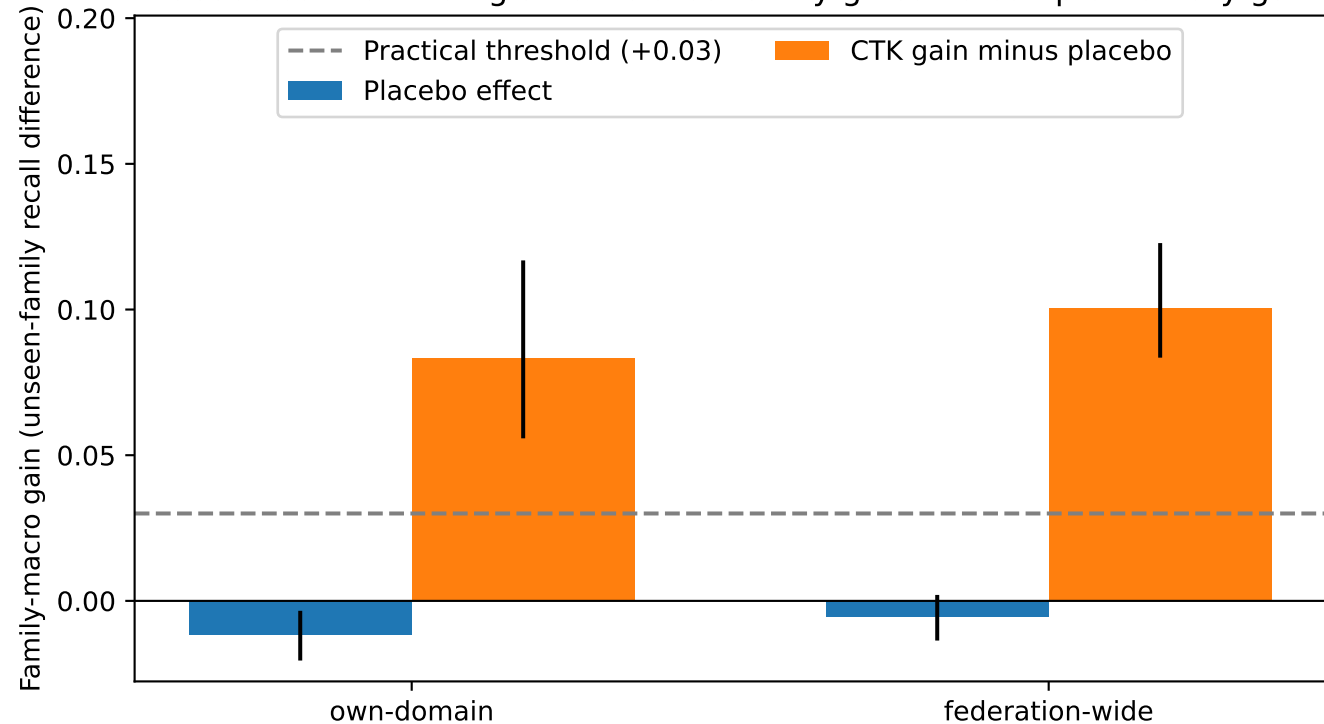
Placebo control: hiding an unrelated family gives no complementary gain
