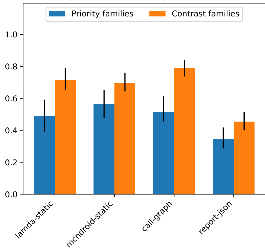
Central full-exposure recall (family-macro, federation-wide)
