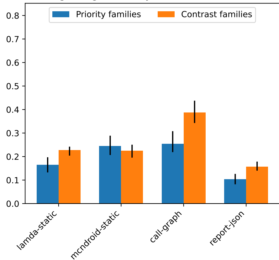
FedAvg CTK gain (family-macro, federation-wide)
