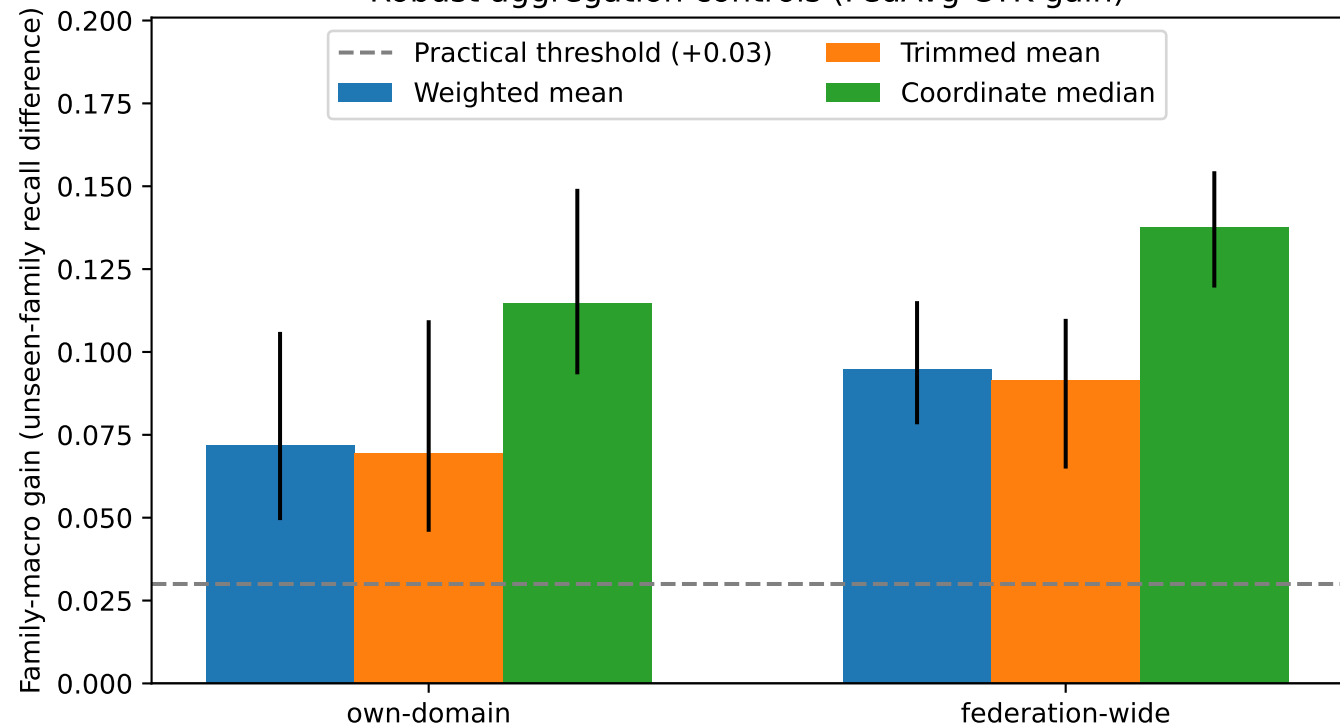
Robust aggregation controls (FedAvg CTK gain)
