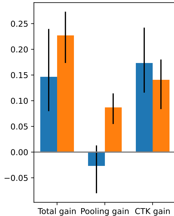
worst-client-unseen-recall
