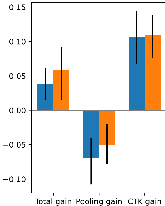
own-domain-unseen-recall
