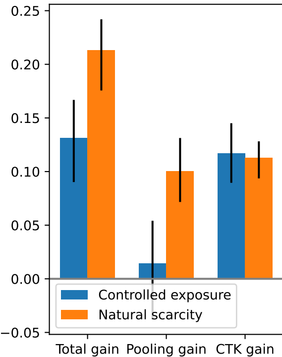
federation-unseen-recall
