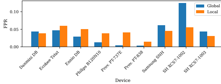
Fig. 2. Per-client FPR under clean baseline, GLOBAL vs. LOCAL threshold (seed 0; CV(FPR) values across all 10 seeds reported in Table 2). GLOBAL forces a single threshold on nine devices with heterogeneous score distributions, producing CV(FPR) = 0.87 for seed 0 (mean = 0.905 \pm 0.039 across seeds). LOCAL fits each client’s own calibration distribution, achieving CV(FPR) = 0.33 on average. CLUSTER is omitted here; its baseline is in Table 2 (CV(FPR) = 0.615 \pm 0.143 ).
