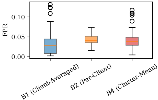
Per-client FPR Distribution (eligible clients, 5 seeds)
