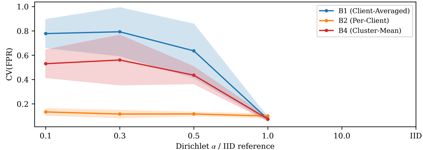
CV(FPR) vs. Dirichlet \alpha (Regime C)
