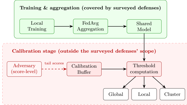
Fig. 1. Attack surface: threshold calibration occurs after FL training. Green boxes mark training and aggregation; the dashed red region marks calibration, outside the scope of the defenses surveyed in Section 2. The three policy nodes are alternative computations, not deployment components; score-level access to one client’s calibration buffer can shift the resulting threshold(s) without modifying model weights, gradients, or labels.
