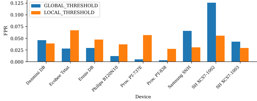
Fig. 2. Clean per-client FPR under Global and Local for seed 4, selected as the lower-median Global CV(FPR) among all 20 seeds using clean metrics only. All-seed estimates appear in Table 2.
