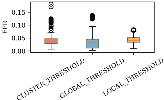
Per-client FPR Distribution (eligible clients, 20 seeds)
