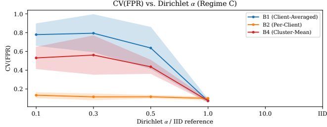
Fig. 4. Regime C: mean CV(FPR) by threshold strategy as a function of Dirichlet \alpha . Whiskers show \pm 1 std over 5 seeds. The B1–B2 gap is largest in the low- \alpha band and disappears under IID or near-homogeneous conditions.
