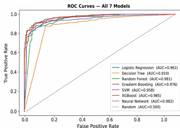
Figure 3 ROC curves for all models
