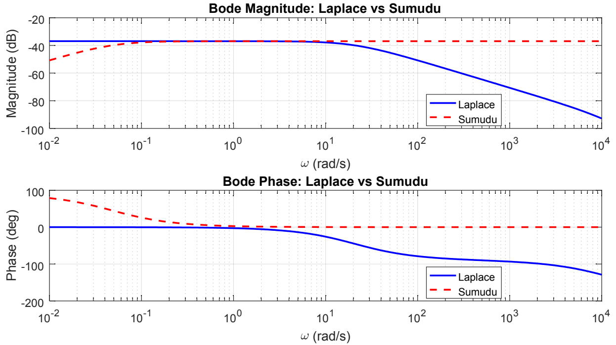
Figure (3) – Bode of Magnitude and Phase for Laplace and Sumudu Transforms
