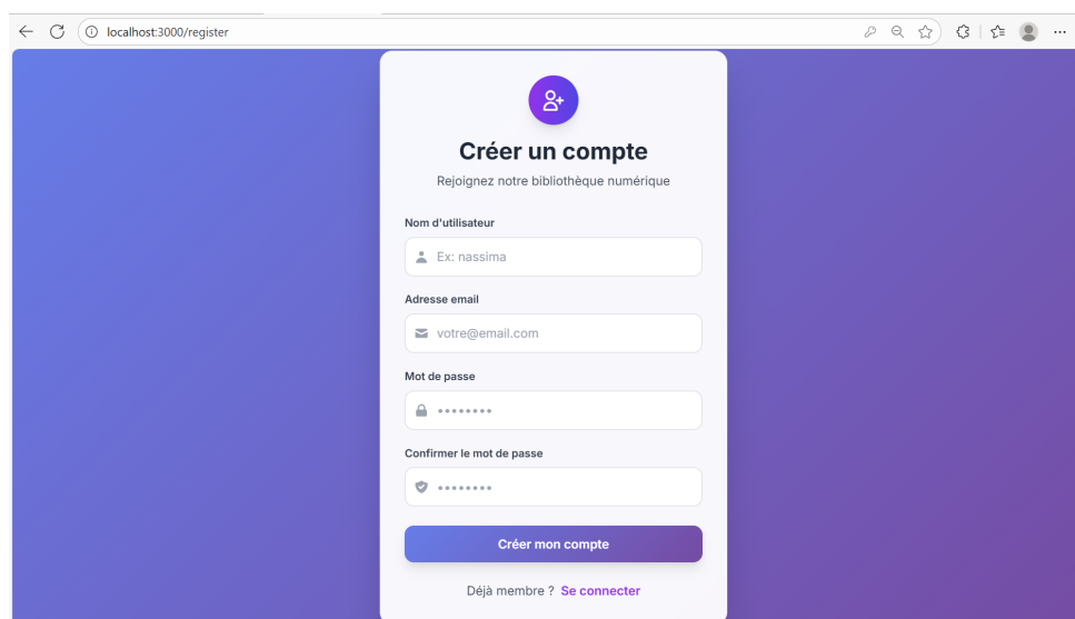
Listing 5 – views/register.pug
