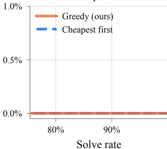
DeepSWE
