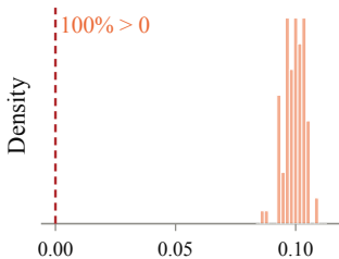
MATH
