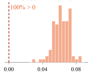
Global-MMLU-Lite
