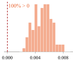
CodeContests
