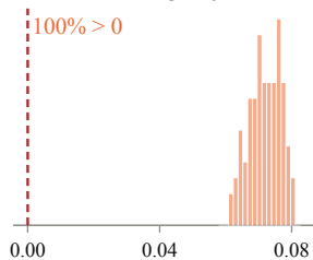
MMLU-Pro
