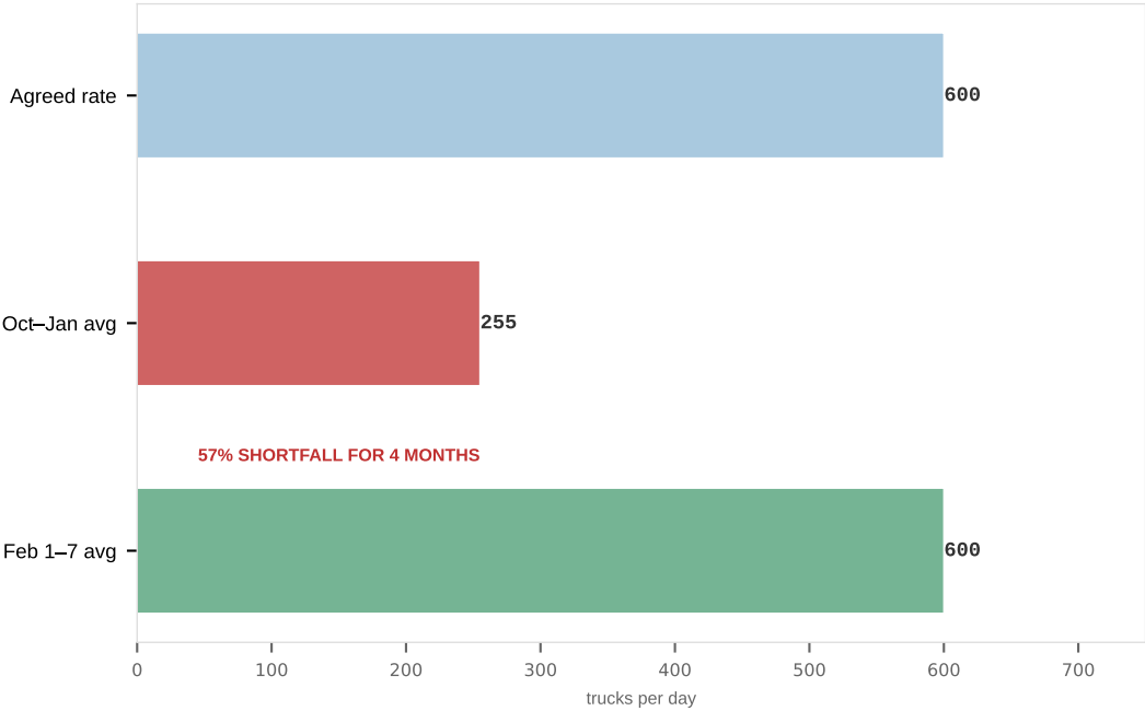
DAILY AID TRUCKS ENTERING GAZA
