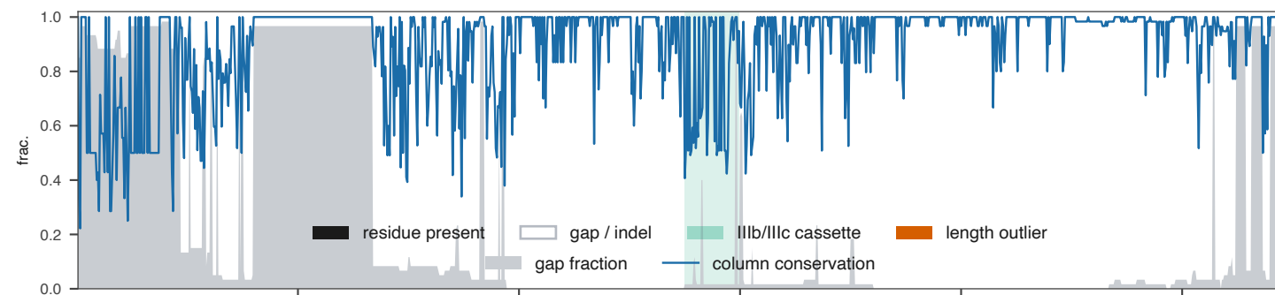
Full-length FGFR2 protein MSA integrity (primary sequences; green band = IIIb/IIIc cassette)
