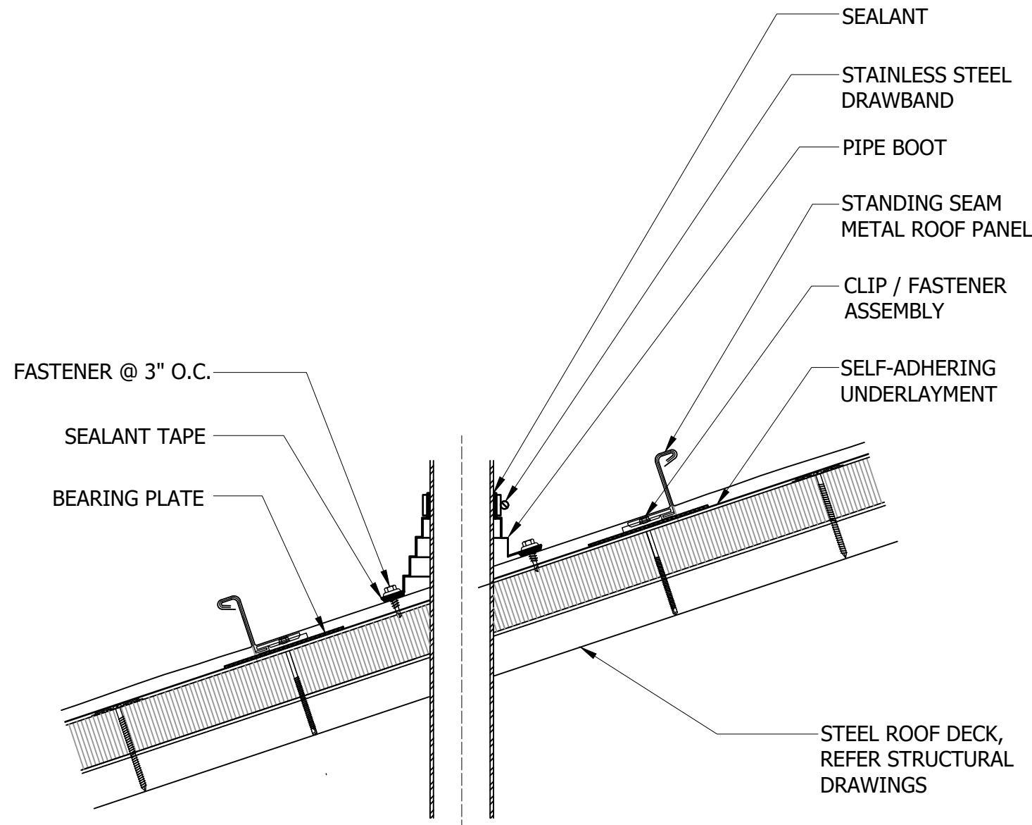
5 PIPE PENETRATION DETAIL C-303 SCALE: NTS
