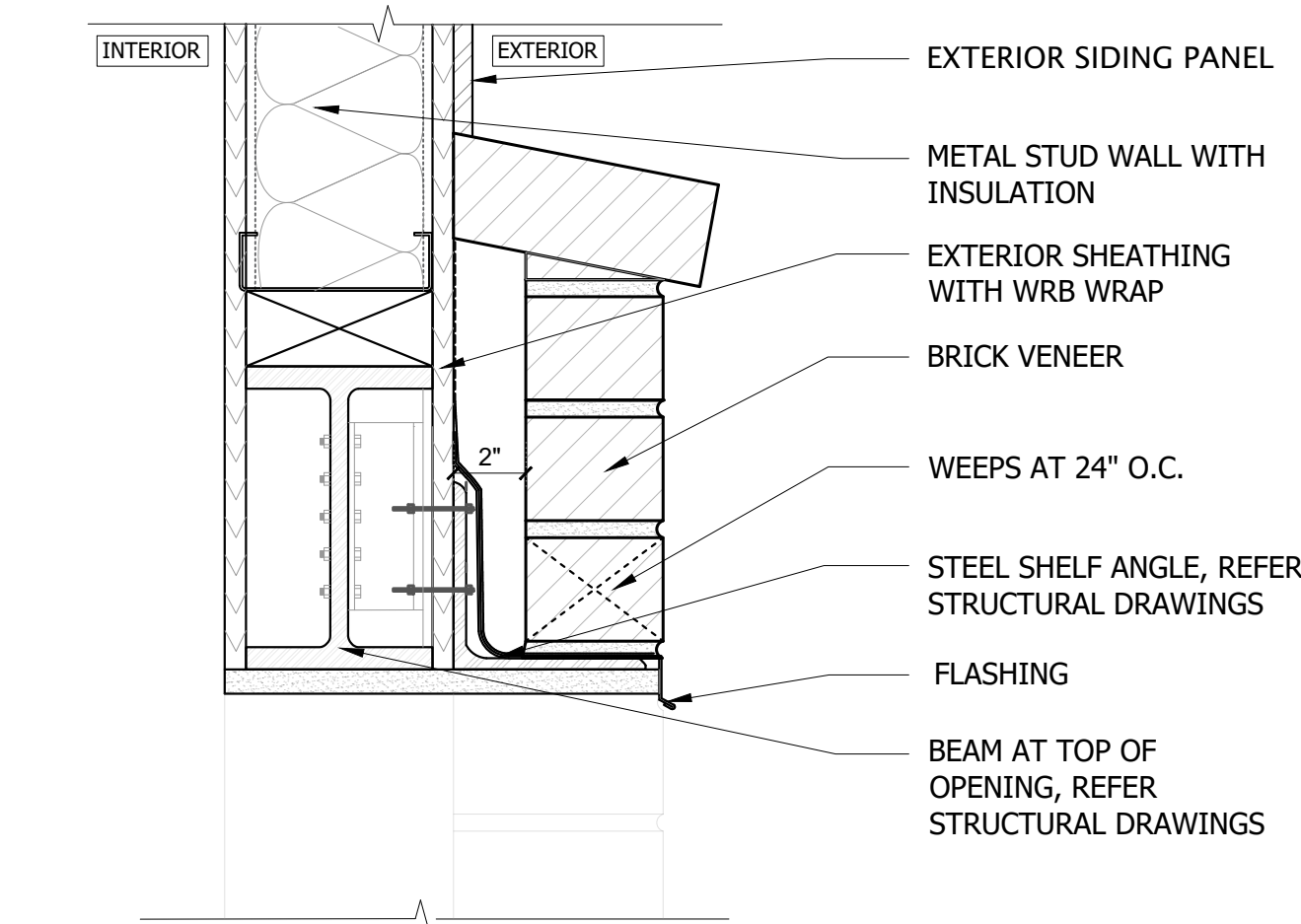
1 OPENING HEAD @ METAL STUD-BRICK C-303 SCALE: NTS
