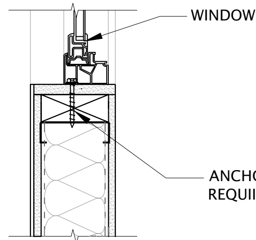
DETAIL- WINDOW (HEAD/JAMB) SCALE: NA
