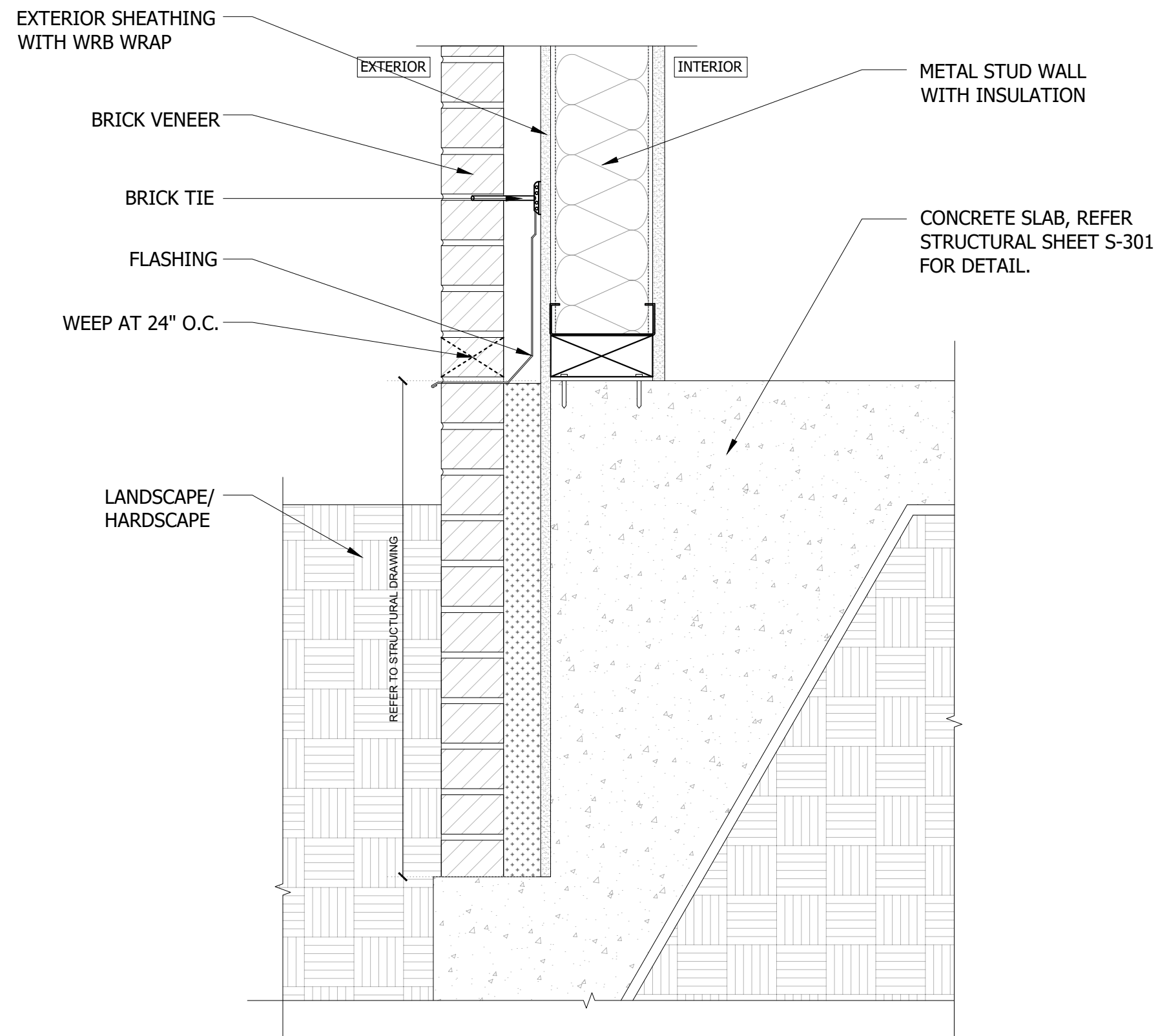
8 BRICK LEDGE DETAIL C-303 SCALE: NTS
