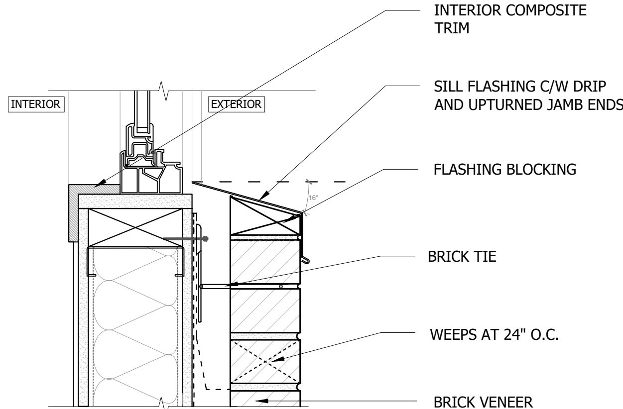
2 WINDOW SILL @ METAL STUD-BRICK C-303 SCALE: NTS
