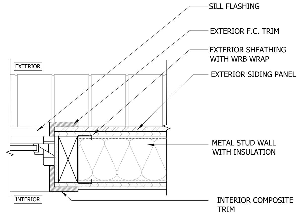
4 WINDOW JAMB AT METAL STUD-F.C. PANEL WITH TRIM C-303 SCALE: NTS
