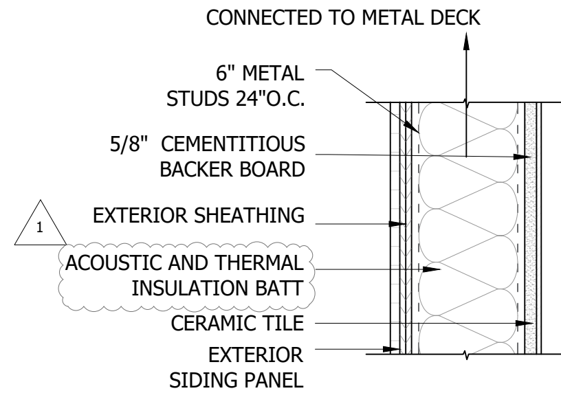
6" PARTITION WALL TYPE B3 SCALE: NTS
