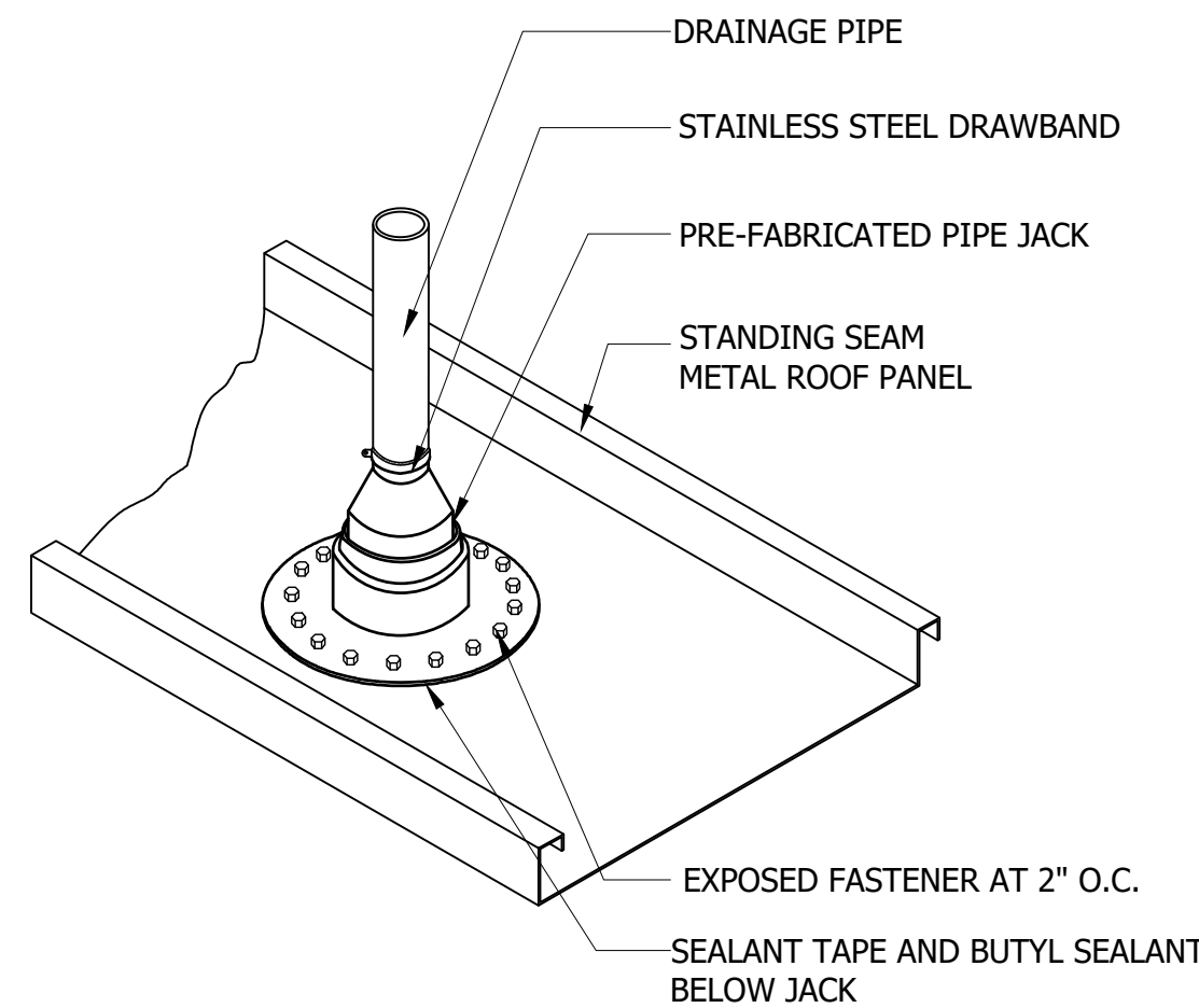
6 PIPE PENETRATION C-303 SCALE: NTS
