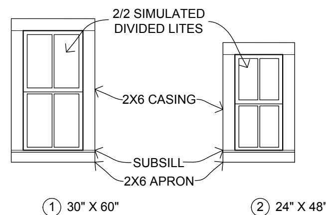
6 WINDOW ELEVATION DETAILS SCALE: 1/4" = 1'-0"
